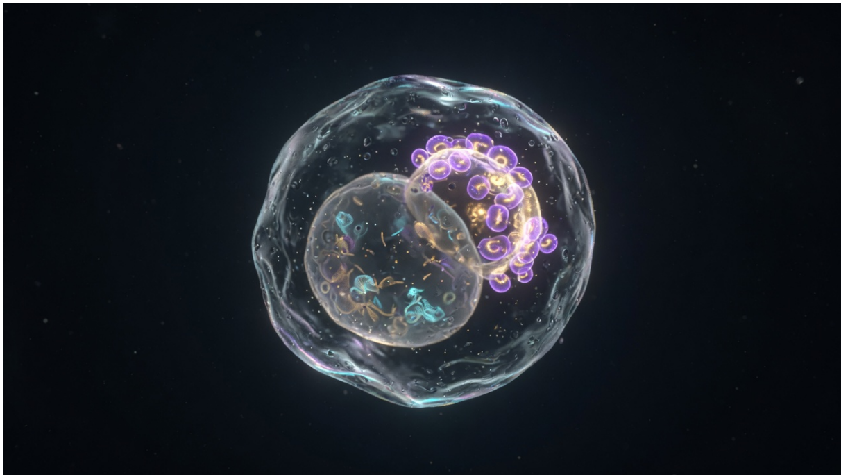
Fig. 8. One pluripotent cell, the opening frame of the machinery film.
