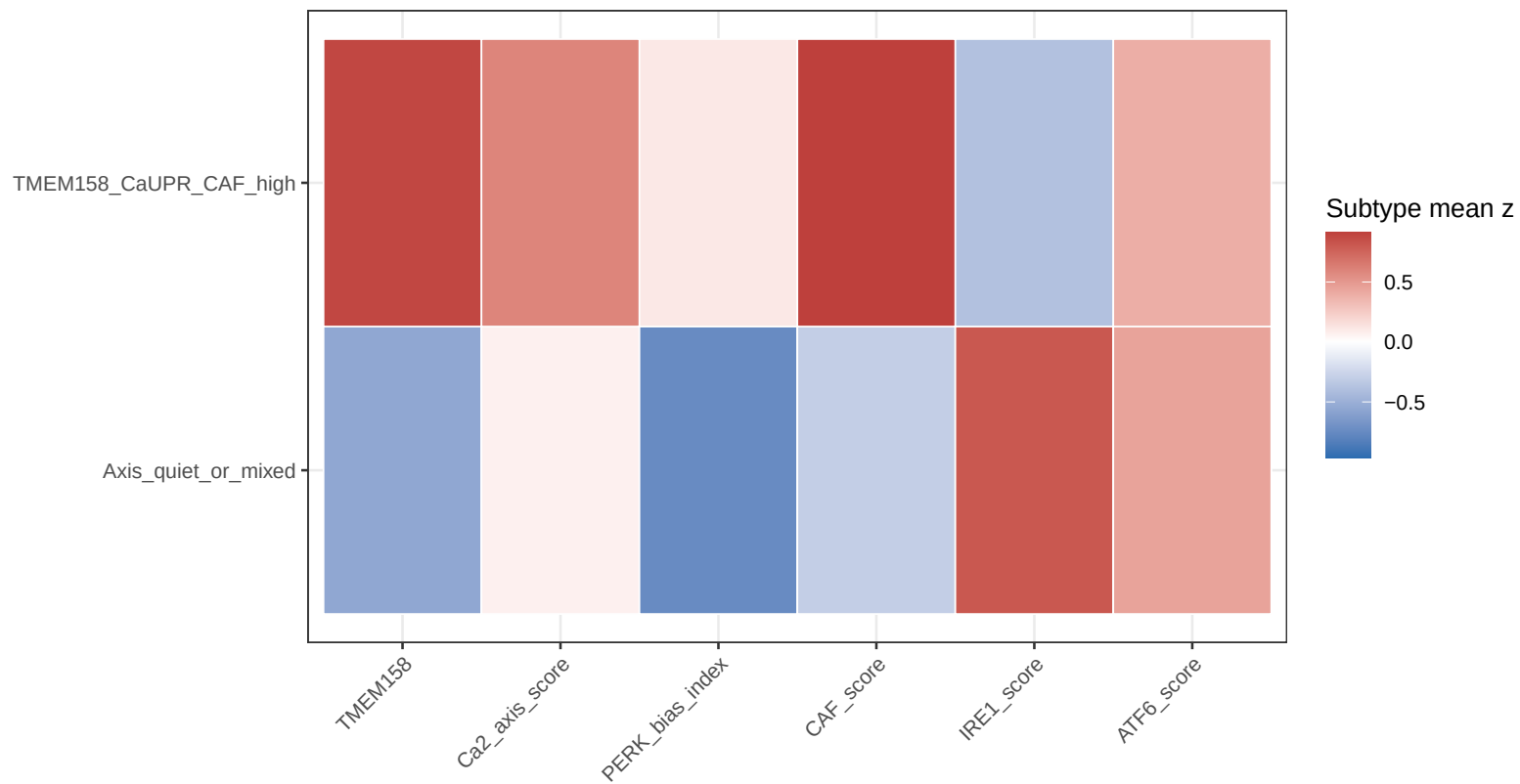
TCGA TMEM158-CaUPR-CAF state subtypes
