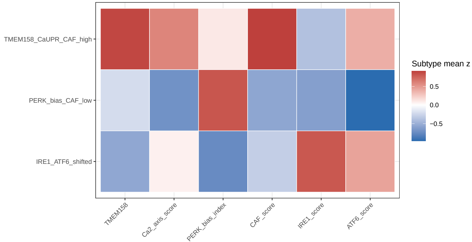
Exploratory TCGA k-means state architecture
