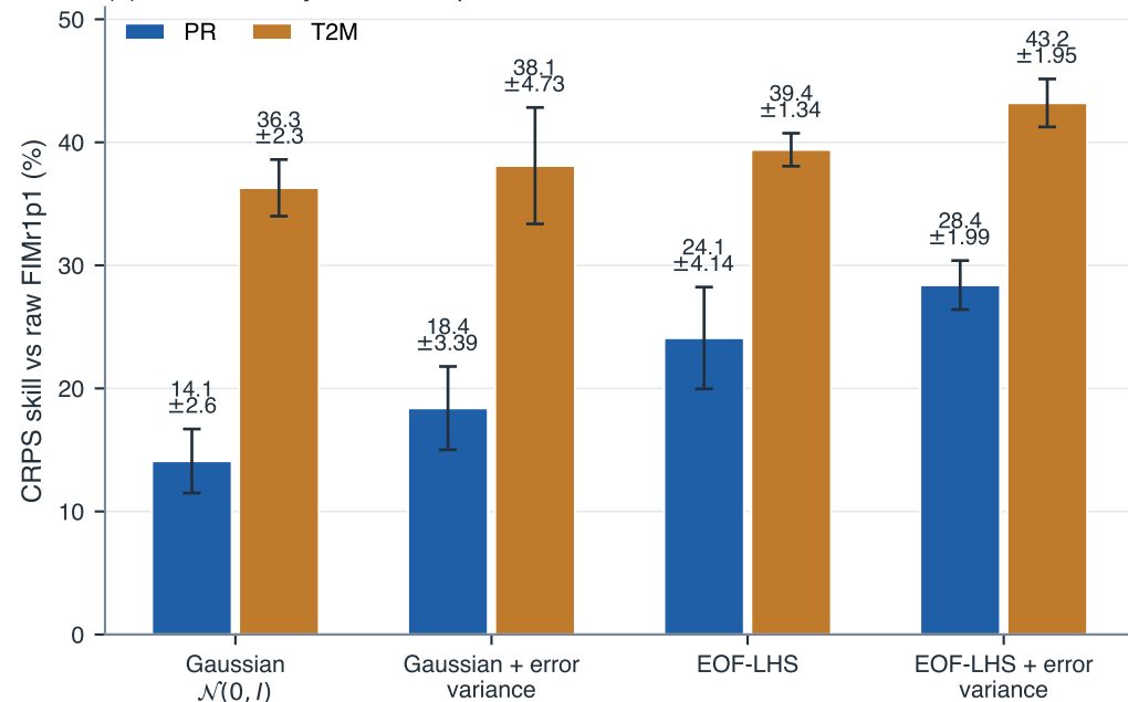
(a) CRPS skill by stochastic prior
