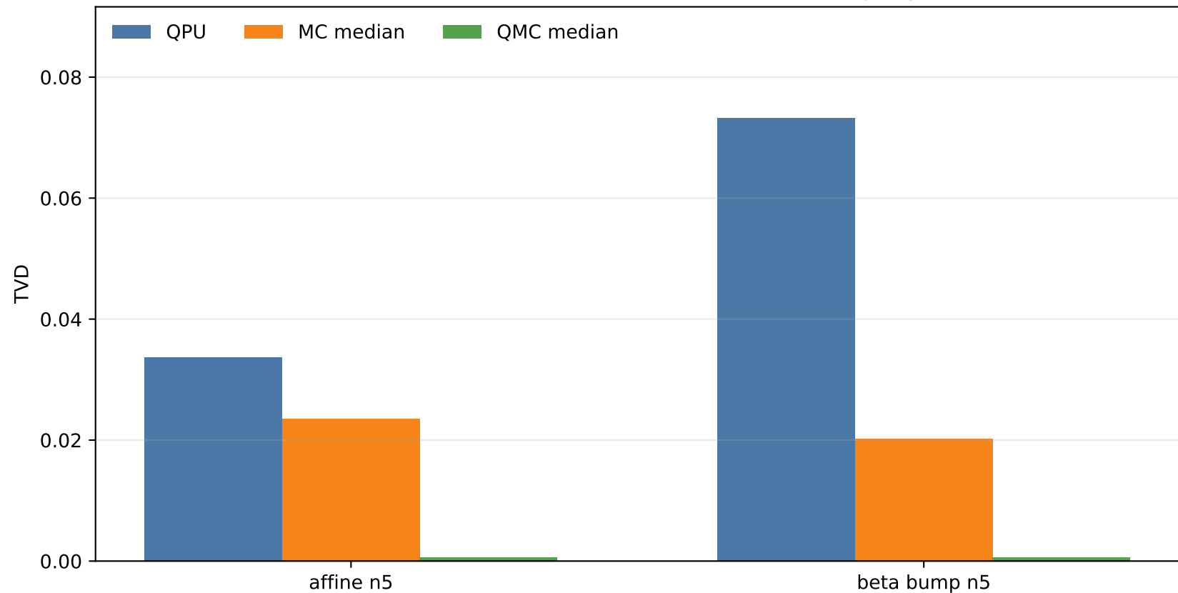
Phase 10 Distribution Error vs Classical Sampling
