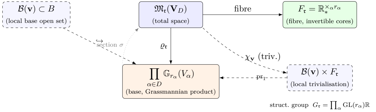
Figure 8.1: Fibre bundle structure of the Tucker manifold \mathfrak{M}_r(\mathbf{V}_D) (Theorem 8.3.2(ii)). The total space projects via \varrho_r onto the base \prod_{\alpha} \mathbb{G}_{r_{\alpha}}(V_{\alpha}) (product of Grassmann–Banach manifolds). Over each chart \mathcal{B}(\mathbf{v}) in the base, the bundle trivialises via \chi_{\mathbf{v}} to a product with the fibre of invertible core tensors F_r . The structure group G_r = \prod_{\alpha} \text{GL}(r_{\alpha})\mathbb{R} acts by change of basis in each minimal subspace. A (local) section \sigma of the bundle corresponds to a chart map \xi_{\mathbf{v}}^{-1} selecting a canonical representative in each fibre.
