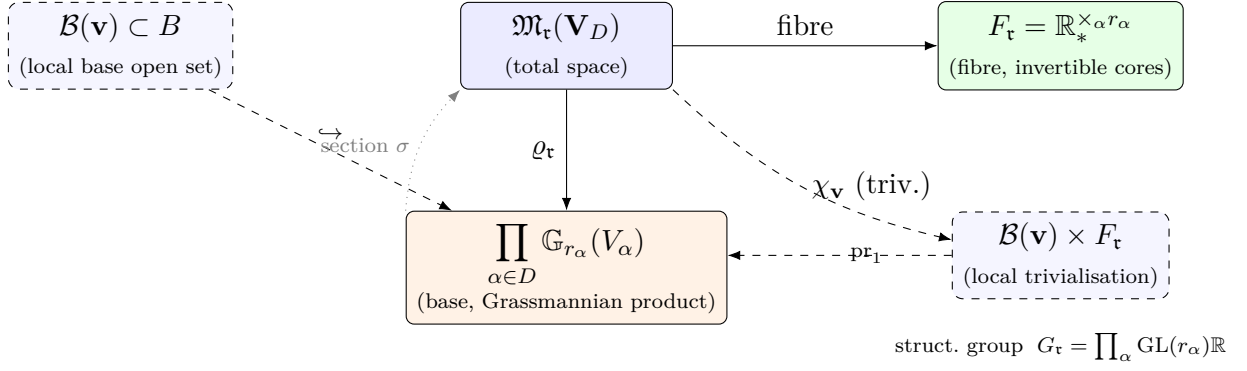
Figure 8.1: Fibre bundle structure of the Tucker manifold \mathfrak{M}_{\mathfrak{r}}(\mathbf{V}_D) (Theorem 8.3.2(ii)). The total space projects via \varrho_{\mathfrak{r}} onto the base \prod_{\alpha} \mathbb{G}_{r_{\alpha}}(V_{\alpha}) (product of Grassmann–Banach manifolds). Over each chart \mathcal{B}(\mathbf{v}) in the base, the bundle trivialises via \chi_{\mathbf{v}} to a product with the fibre of invertible core tensors F_{\mathfrak{r}} . The structure group G_{\mathfrak{r}} = \prod_{\alpha} \text{GL}(r_{\alpha})\mathbb{R} acts by change of basis in each minimal subspace. A (local) section \sigma of the bundle corresponds to a chart map \xi_{\mathbf{v}}^{-1} selecting a canonical representative in each fibre.
