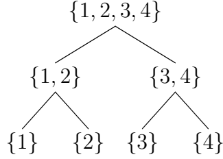
Figure 5.2: Balanced binary tree over D = \{1, 2, 3, 4\} : depth 2, corresponding to the HT format.
