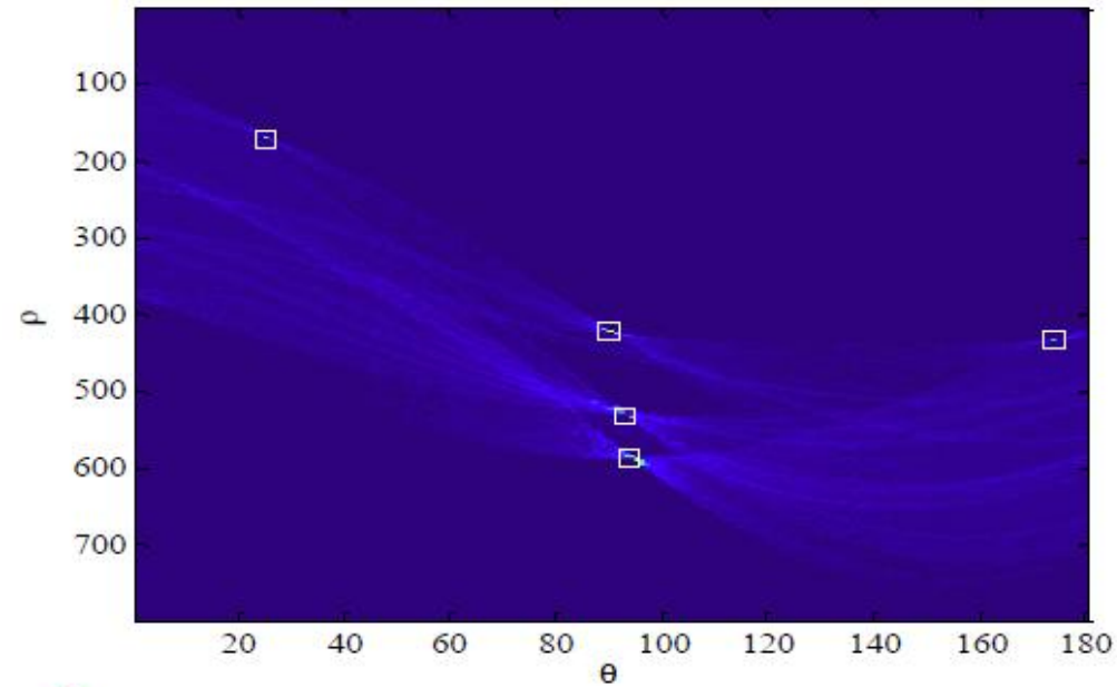
Hough Transform
