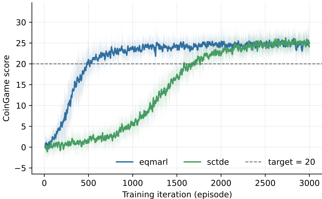
Ideal learning curves
