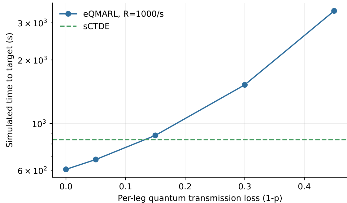
Time-to-target versus loss
