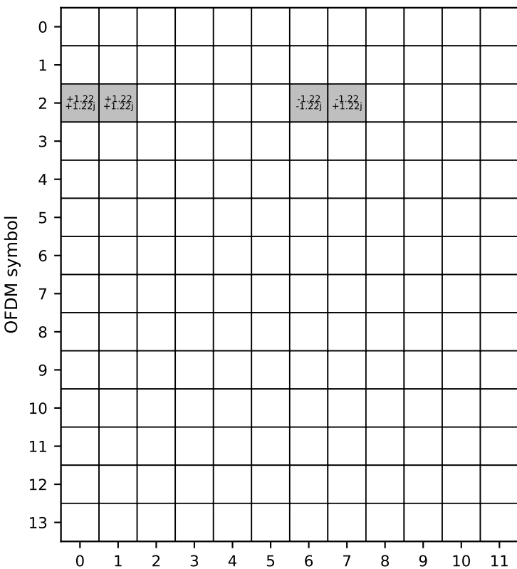
User 3 DMRS port set=[2]
