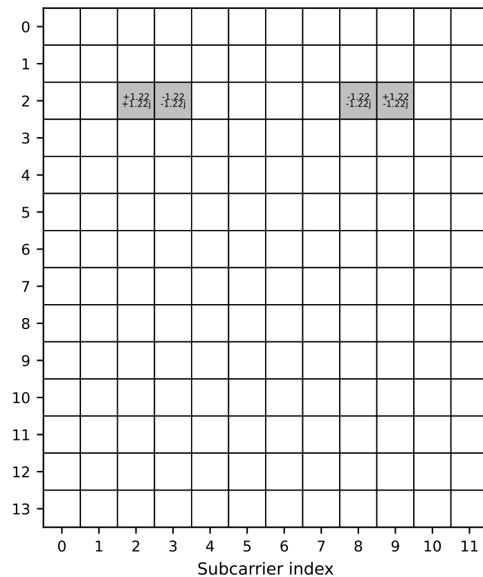
User 4 DMRS port set=[3]
