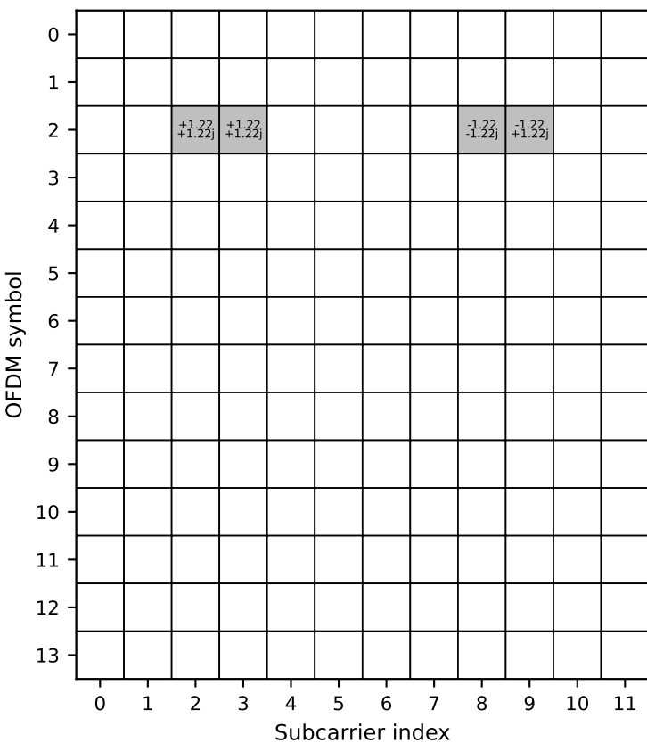
User 3 DMRS port set=[2]
