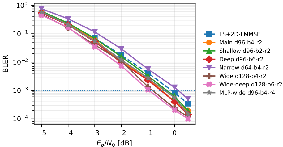
BLER crossing used for SNR-gain table
