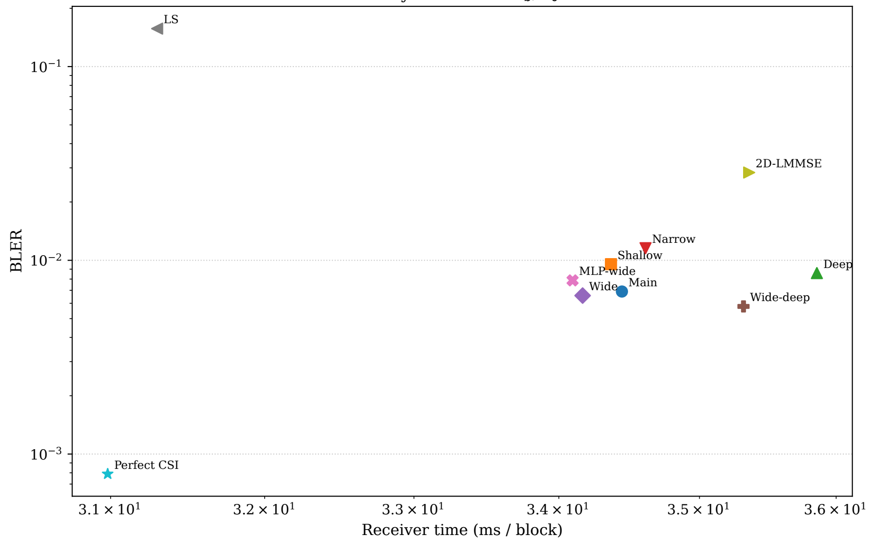
BLER-latency tradeoff at E_b/N_0 = -2 dB
