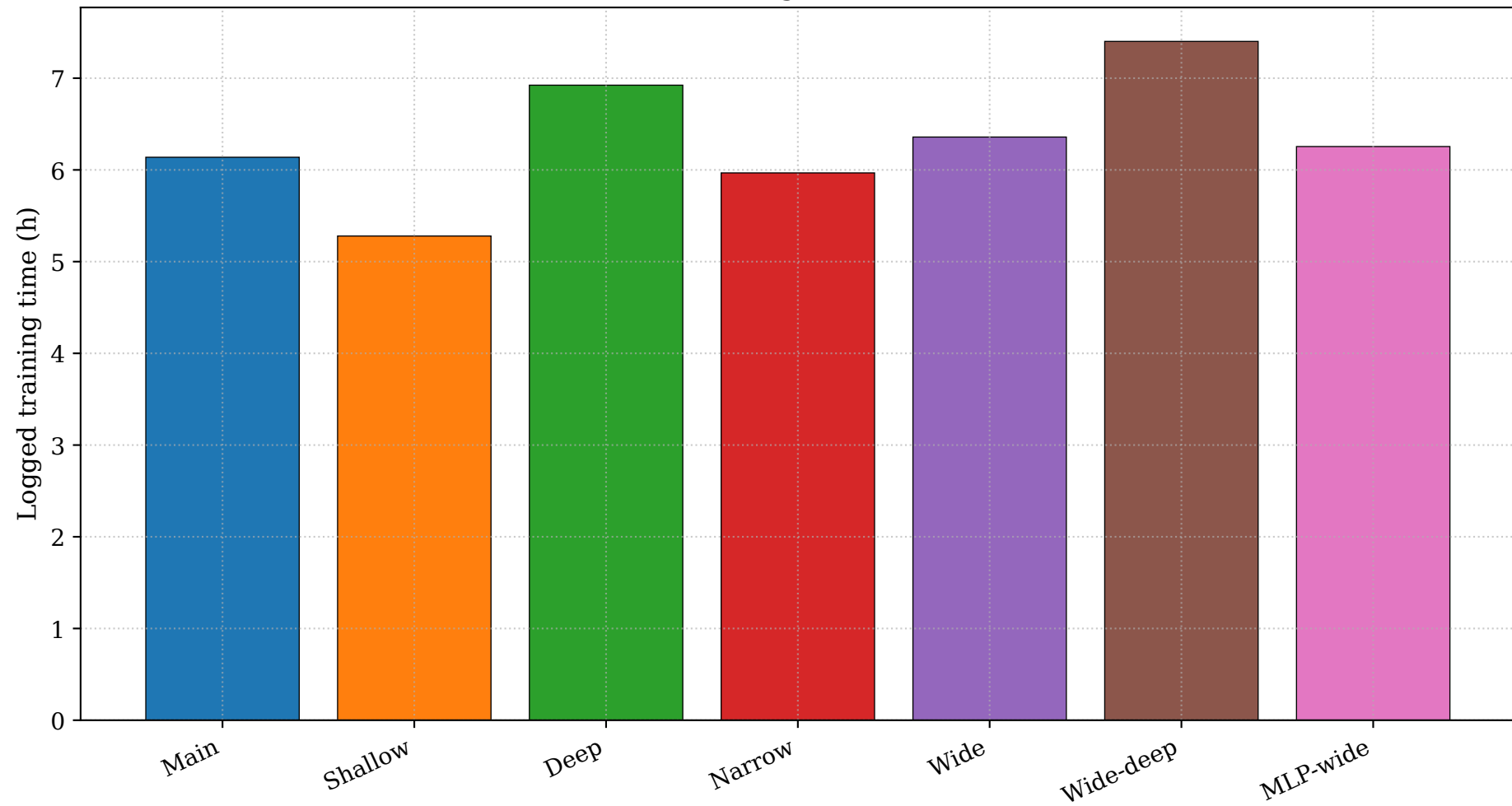
Training runtime
