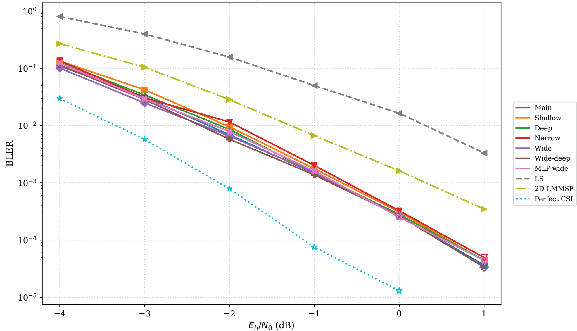
BLER comparison (3 users)
