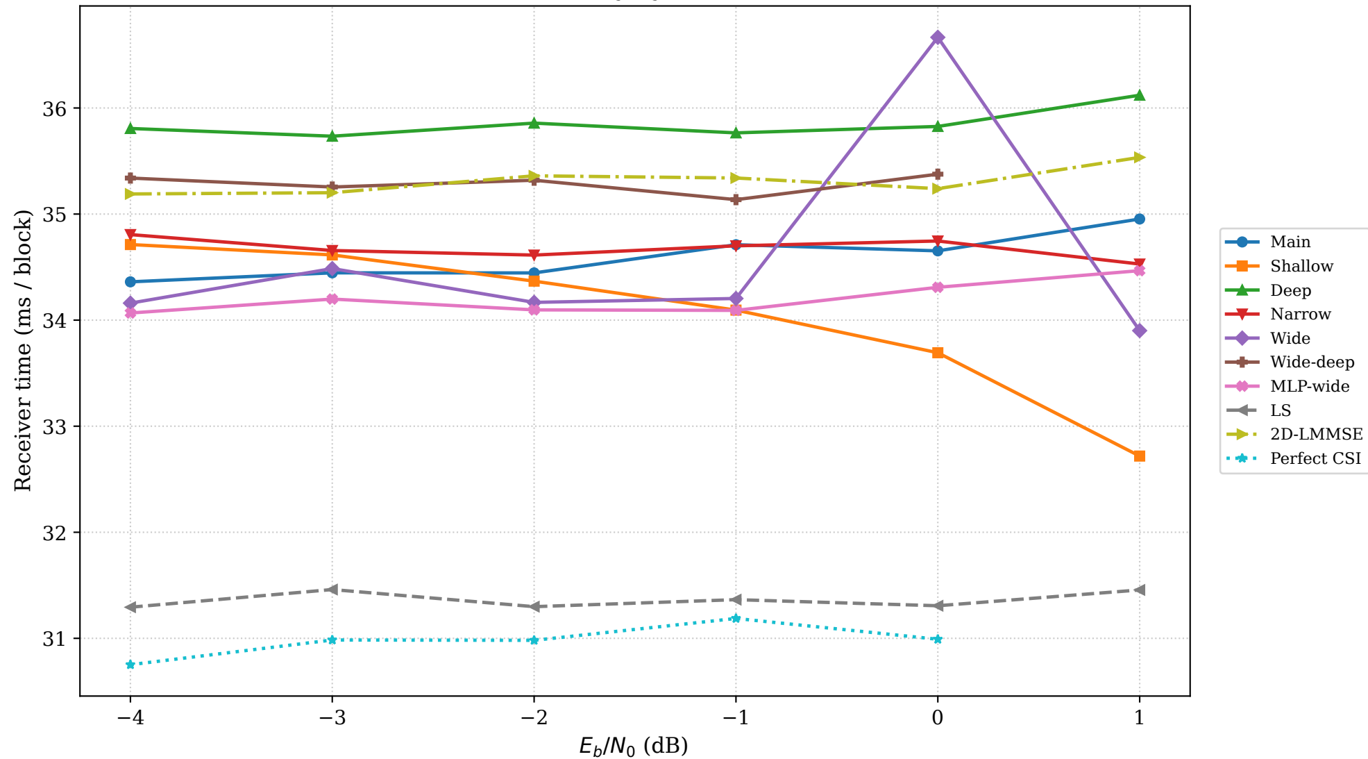
Receiver latency by SNR (3 users)
