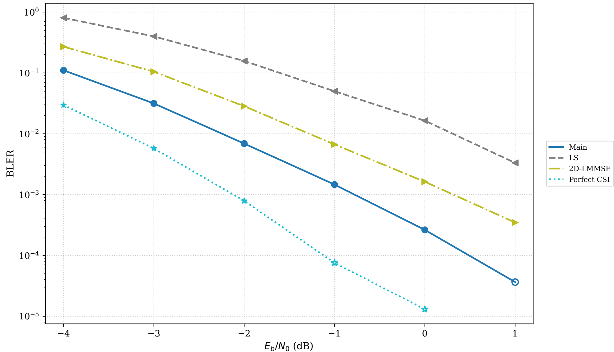
Main UPAIR vs benchmarks (3 users)
