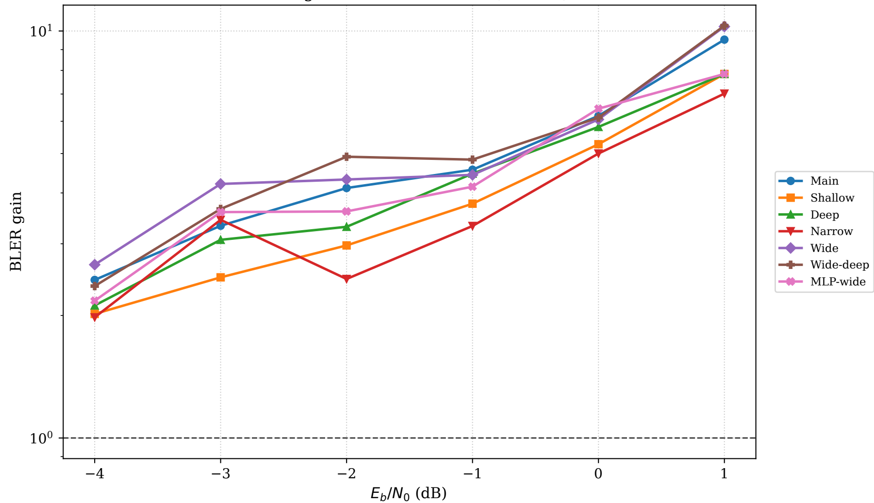
BLER gain over 2D-LMMSE (3 users)
