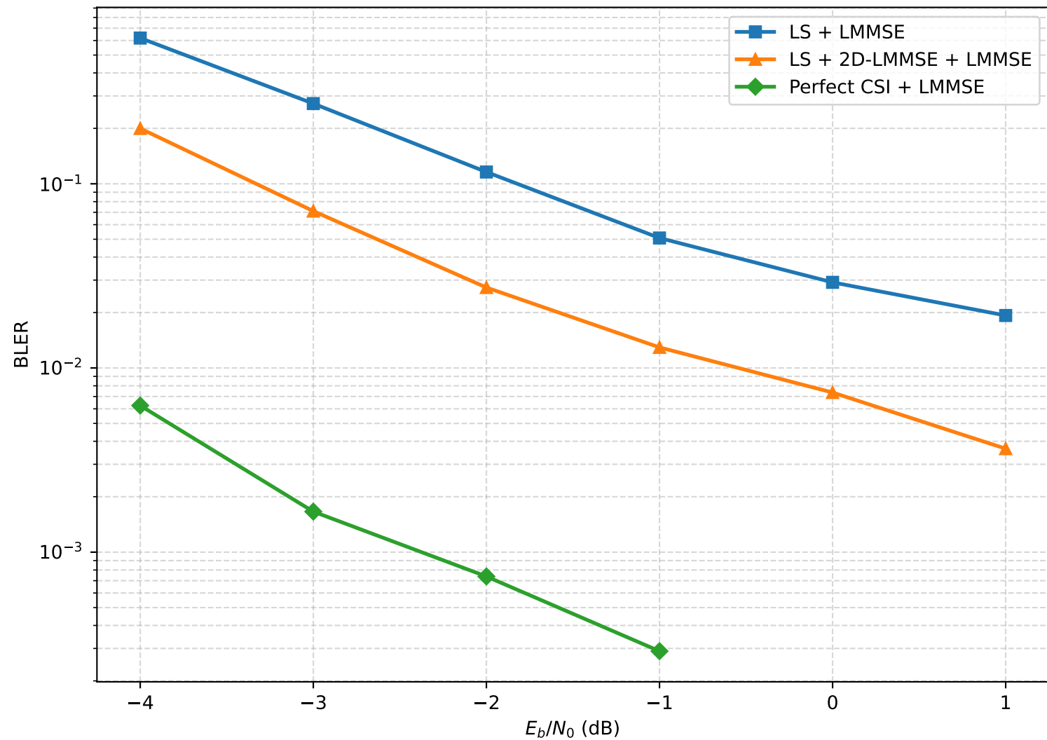
UMi, U=3: UPAIR Main vs Baselines
