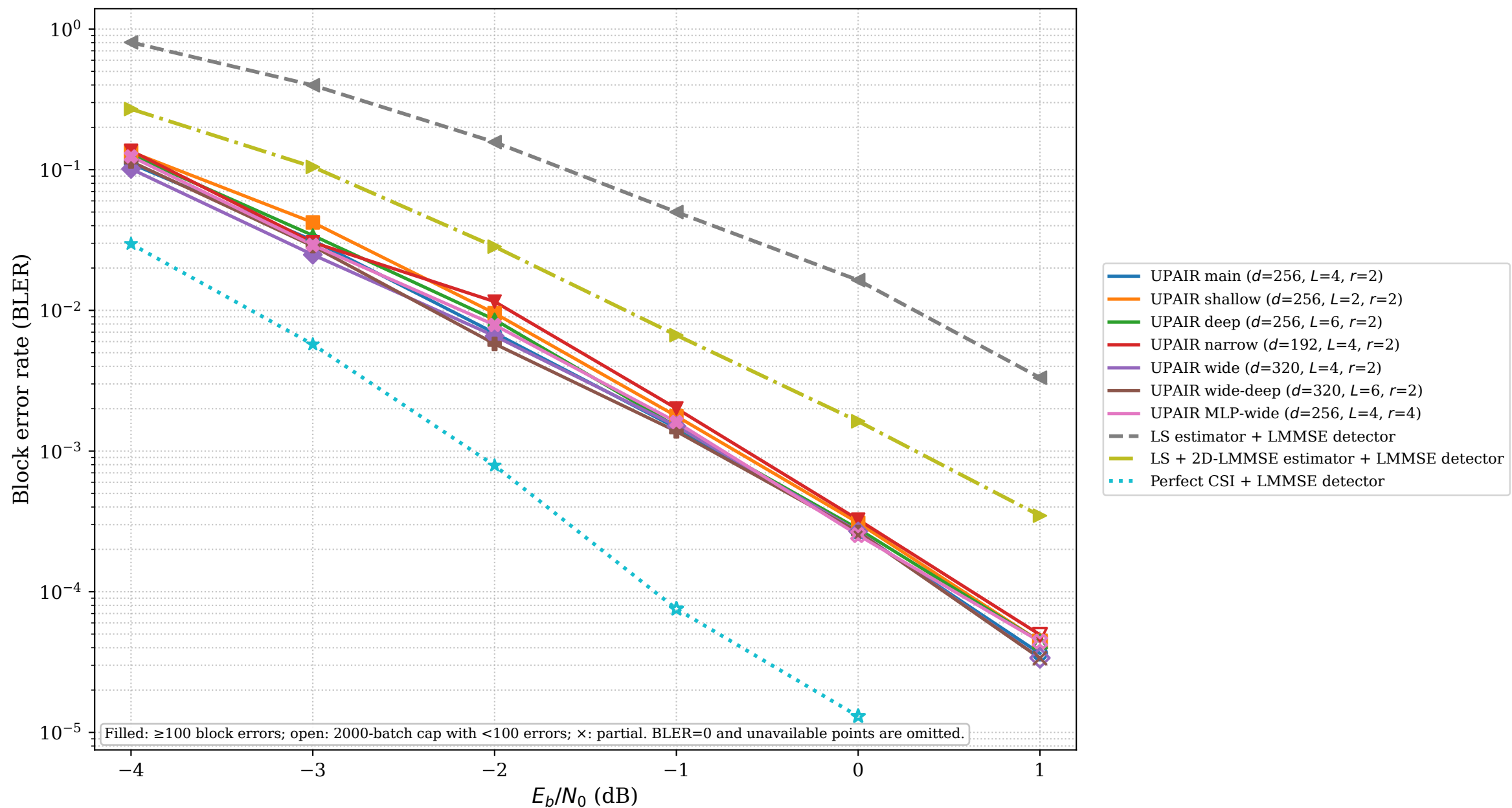
Extended UPAIR architecture variants and receiver benchmarks 3 active users
