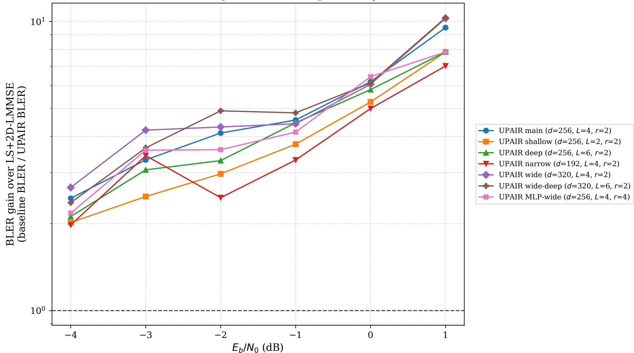
Extended UPAIR gain relative to LS+2D-LMMSE 3 active users; positive common points only
