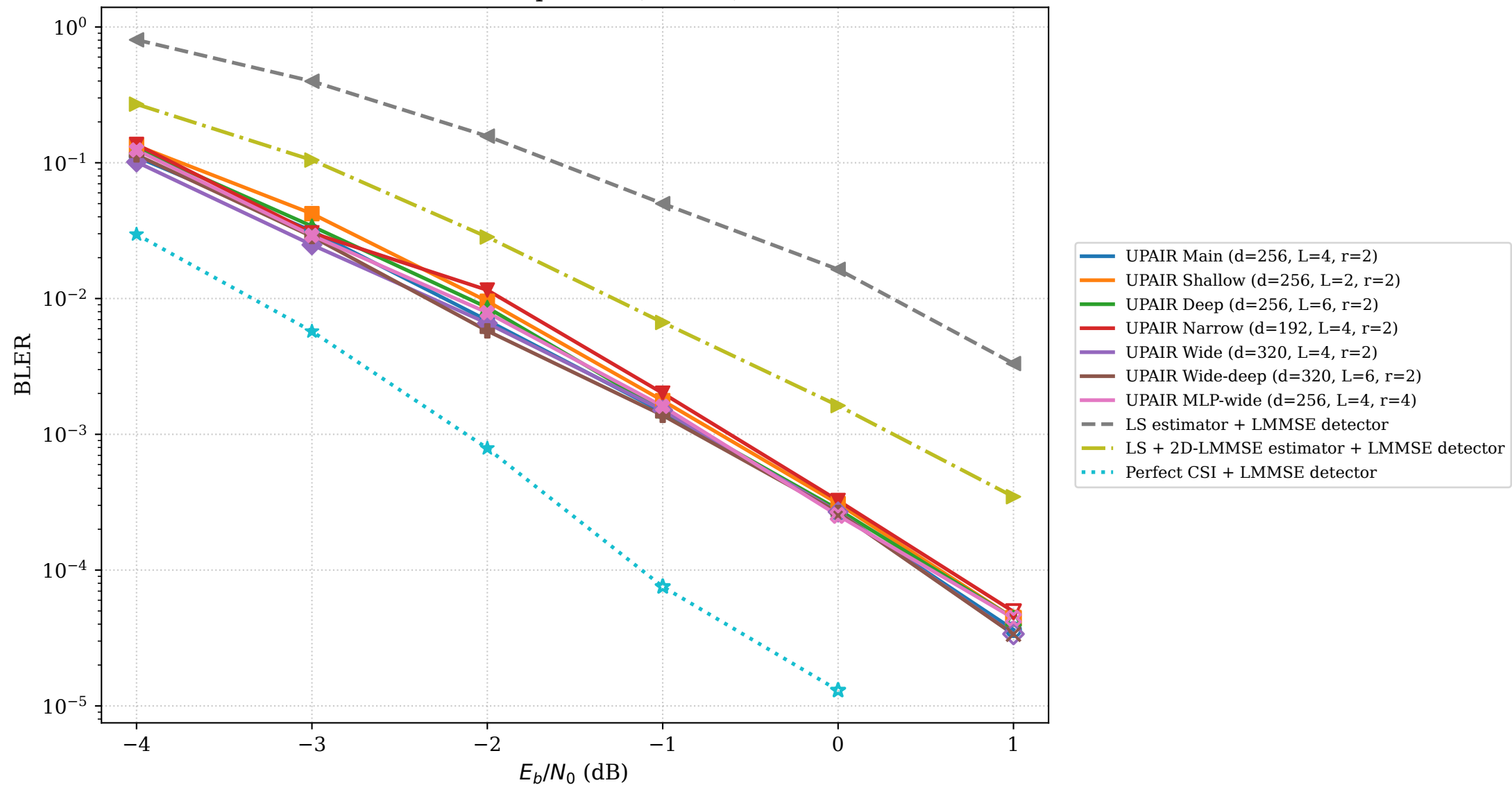
BLER comparison (3 users)
