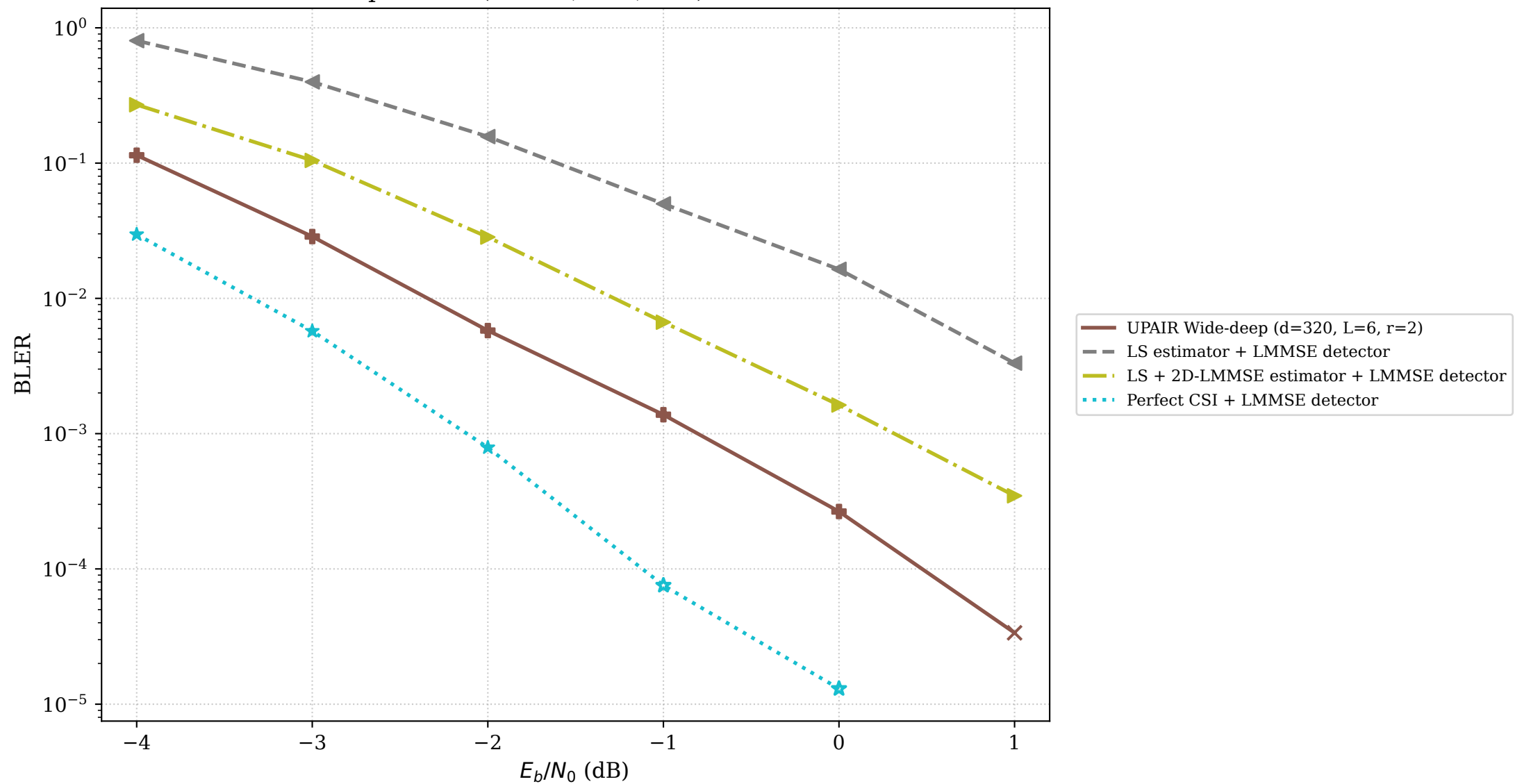
Wide-deep UPAIR ( d=320 , L=6 , r=2 ) vs benchmarks
