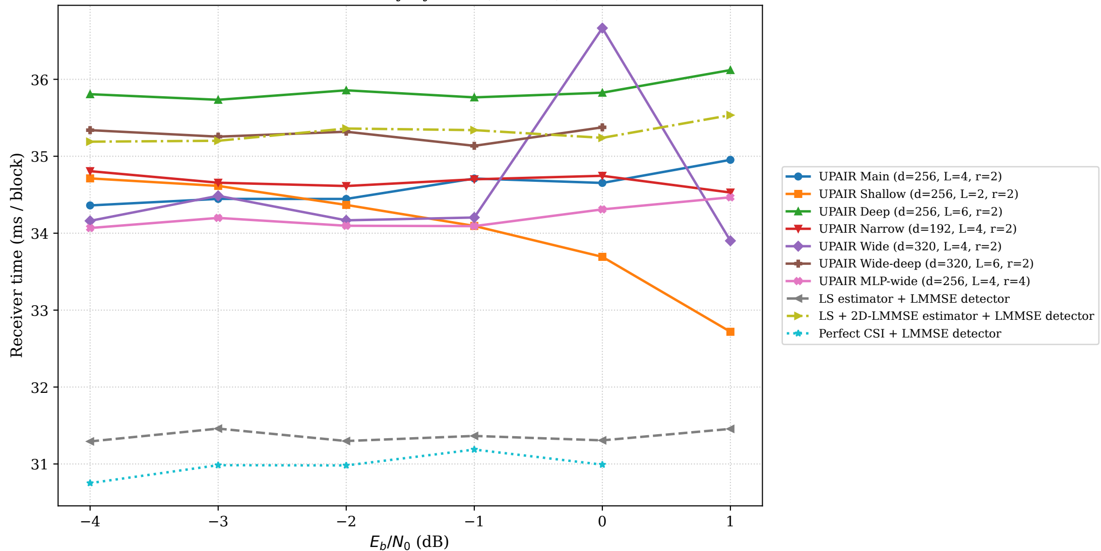
Receiver latency by SNR (3 users)
