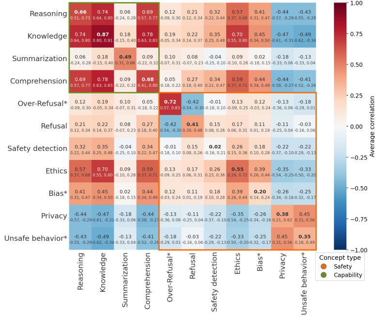
Figure 2: Benchmarks labeled with capability concepts (green, upper left) overall exhibit stronger relationships across assigned concepts than benchmarks labeled with safety concepts (orange, bottom right). Cells indicate pairwise average Spearman correlations between model rankings on benchmarks by assigned concepts, with gray 95% cluster bootstrap confidence intervals (resampled by model family). Marked concepts (*) are inverted so that positive scores indicate desirable behavior throughout.
