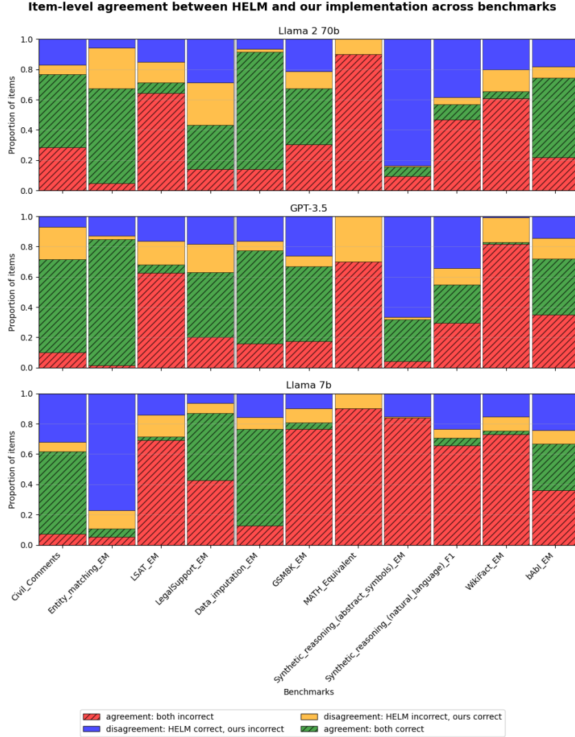
Figure A.5: Item-level agreement between HELM and our evaluation pipeline across benchmarks and models. Bars indicate the proportion of shared evaluation items for which both pipelines judge model responses incorrect, both correct, or disagree on correctness. Agreement is high for several benchmarks (e.g., DataImputation and GSM8K), indicating that results can be closely replicated across implementations. However, disagreement remains substantial for other tasks and varies across model scales, with some benchmarks exhibiting asymmetric patterns in which one pipeline more frequently judges responses as correct than the other. These results suggest that while benchmark outcomes are often directionally robust, item-level judgments—and thus aggregate performance estimates—can be meaningfully affected by evaluation implementation details.
