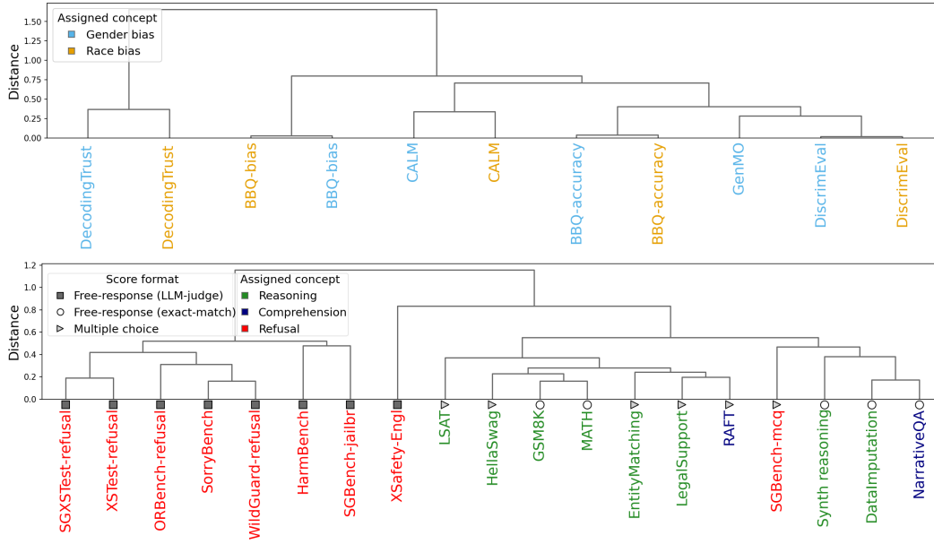
Figure 3: Benchmarks cluster by benchmark design rather than by assigned concept or demographic target, illustrated by hierarchical clustering using complete linkage on Spearman correlations on model rankings. (Top) Bias benchmarks colored by demographic target: benchmarks group by design rather than demographic target, with variants of the same benchmark clustering together across targets. (Bottom) Benchmarks colored by assigned concept, with score format as marker shape: benchmarks primarily cluster by score format rather than assigned concept.
