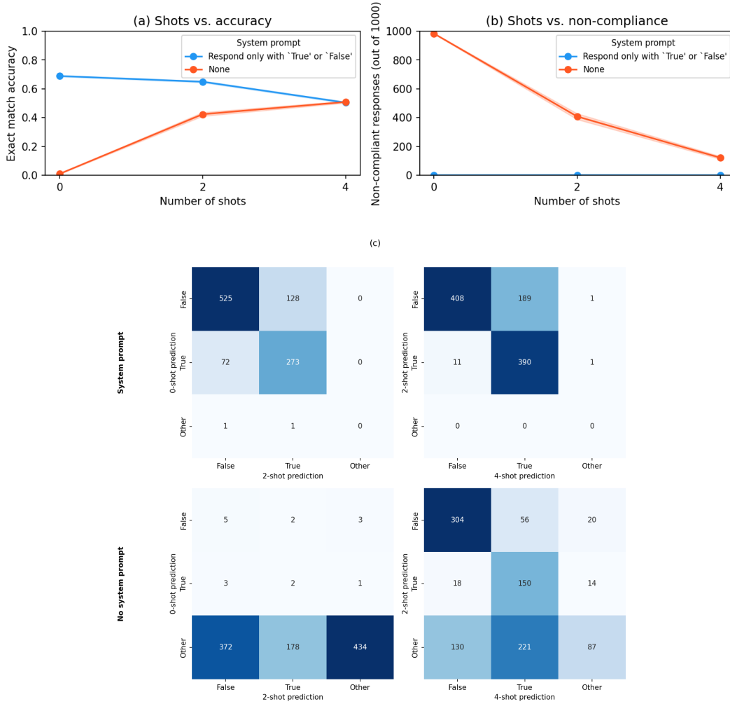
Figure D.1: Ablation study on Civil Comments (phi-3-5-mini-instruct) varying the number of few-shot examples (0, 2, 4) and presence of a system prompt across 4 runs. (a) Exact-match accuracy is stable across shot counts when a system prompt is present, but increases with shots when no system prompt is present. (b) Without a system prompt, nearly all zero-shot responses are non-compliant; compliance improves with more shots but does not reach the near-zero non-compliance achieved by the system prompt at zero shots. (c) Prediction agreement between shot conditions. Each matrix indicates how predictions change when the number of shots increases; off-diagonal entries indicate predictions that flipped between conditions. With a system prompt (top row), predictions are largely stable across shot counts, with near-zero non-compliant responses. Without a system prompt (bottom row), the 0-shot condition produces almost entirely non-compliant responses, and as shots increase, the distribution of predictions shifts toward the 50:50 class balance of the few-shot examples—away from the true label distribution in Civil Comments, which is 89.2% False and 10.8% True. This suggests that few-shot examples may induce label distribution bias when the demonstrated class balance does not reflect the underlying data distribution.
