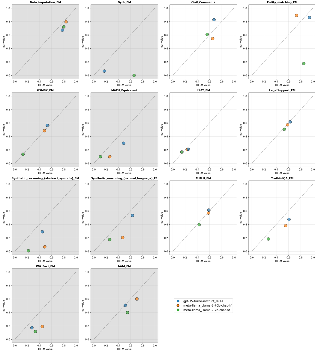
Figure A.4: Comparison of model scores computed in our evaluation pipeline versus reported results from HELM (Liang et al., 2022) for overlapping benchmarks and models. Many benchmarks exhibit near-diagonal agreement, indicating close replication of reported performance (e.g., LegalSupport, GSM8K, MMLU). Where discrepancies arise, model rank ordering is often preserved (e.g., DataImputation and Synthetic Reasoning (Natural)), suggesting that comparative conclusions about model capability can be robust to differences in evaluation implementation. However, agreement is inconsistent across benchmarks, with some tasks indicating substantial divergence in both absolute scores and rank ordering, highlighting the sensitivity of benchmark outcomes to implementation details.
