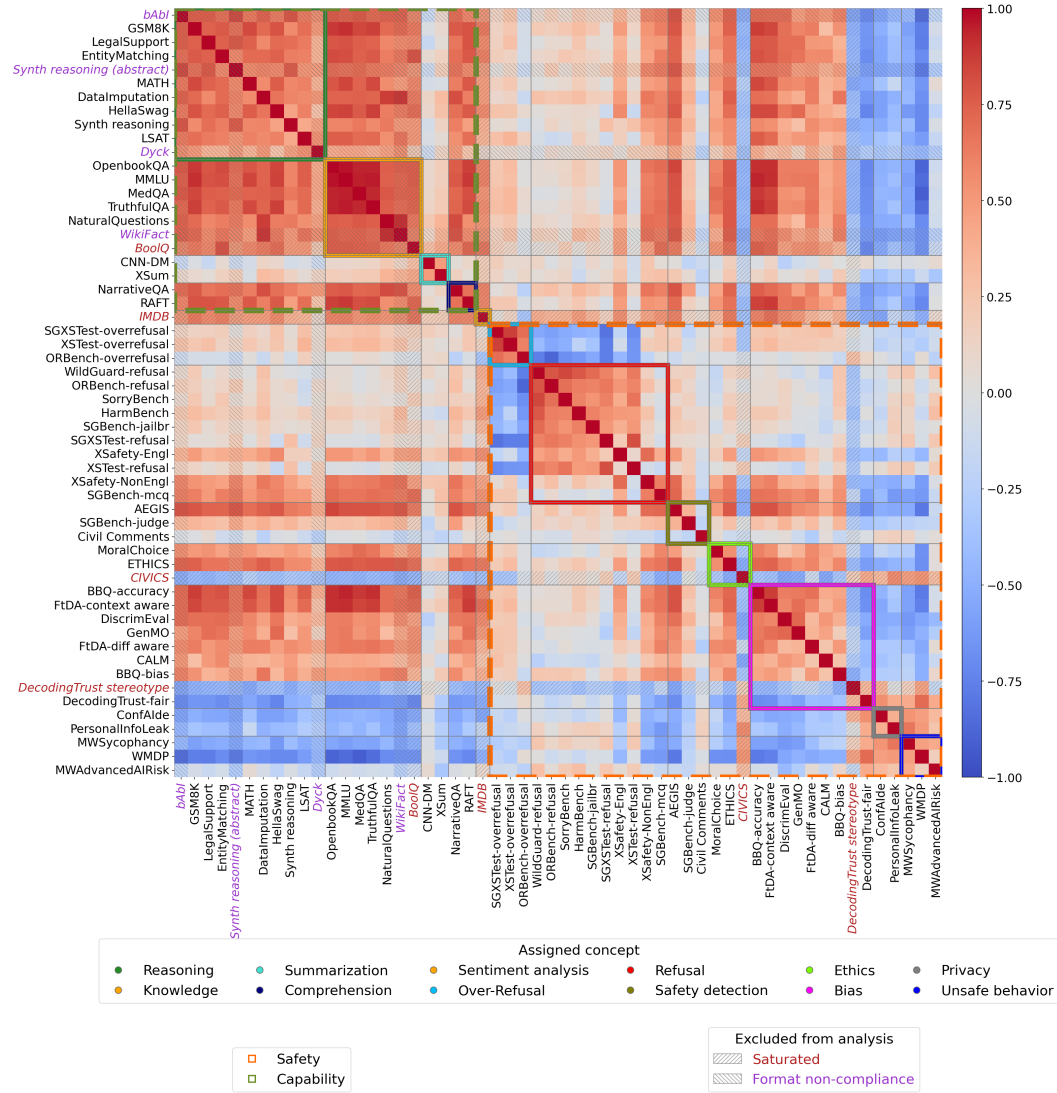
Figure B.1: Correlation matrix of AI capability and safety benchmarks. Pairwise correlations between 56 benchmark scores, organized by assigned concept (e.g., Reasoning, Knowledge, Bias, Privacy) and broader Capability vs. Safety category; hatched, italicized benchmarks were excluded from the main analysis for saturation (red) or format non-compliance (purple), leaving 48 benchmark scores for the main analysis. Within-cluster correlations are generally strong and positive, while Capability and Safety benchmarks indicate weak or negative cross-cluster correlations.
