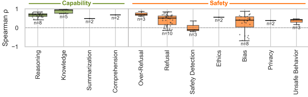
Figure 1: Convergence of benchmarks with the same assigned concept ( n = number of benchmarks per assigned concept). Distributions of pairwise Spearman correlations between model rankings on benchmarks with the same assigned concept; model rankings on benchmarks labeled with capability concepts correlate consistently with one another, while model rankings on benchmarks labeled with safety concepts do not.
