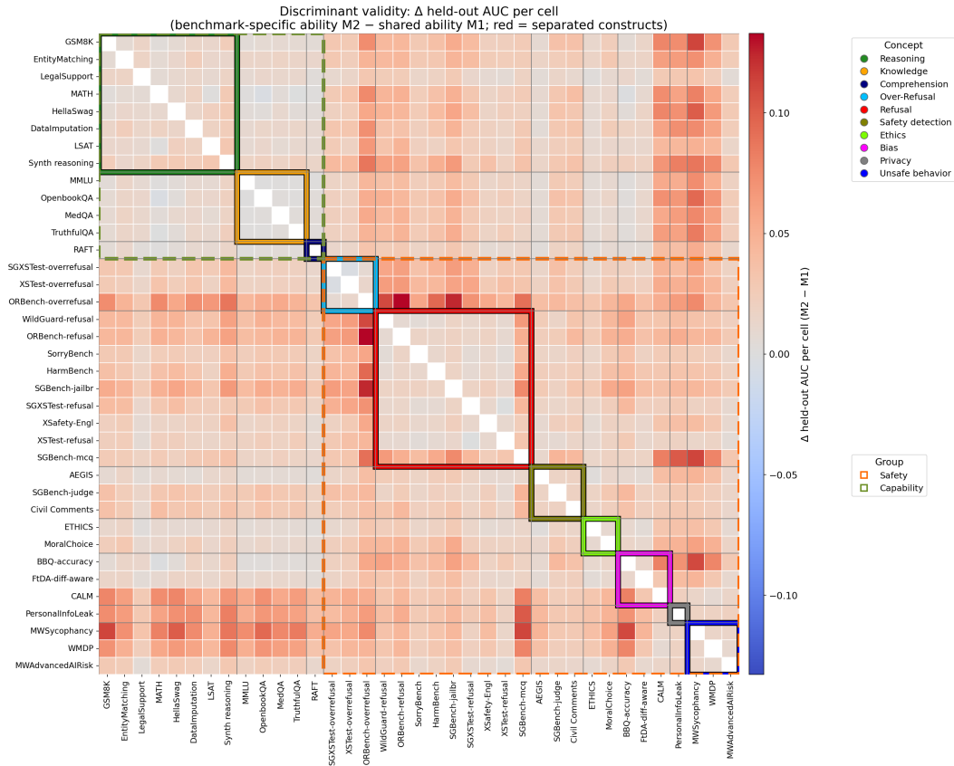
Figure B.2: Pairwise item-level discriminant validity across the 37 IRT-eligible benchmarks: gain in held-out prediction AUC ( \Delta AUC) from fitting each pair benchmark-specific latent traits rather than one ability shared across the pair. Values near zero indicate the pair is well described by a single shared ability; higher (redder) values indicate the pair requires separate, benchmark-specific latent traits.
