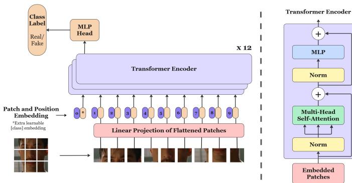
Gambar 3.9 Arsitektur model spasial berbasis Vision Transformer (ViT)
