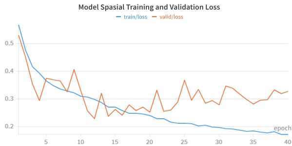
(a) Model spasial
