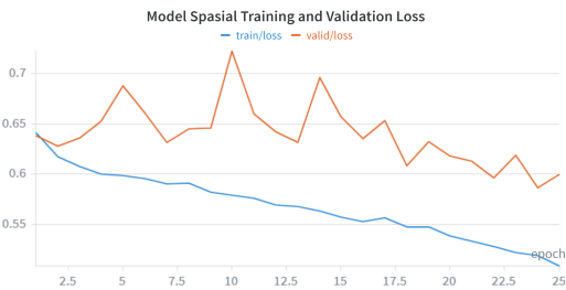
(a) Model spasial
