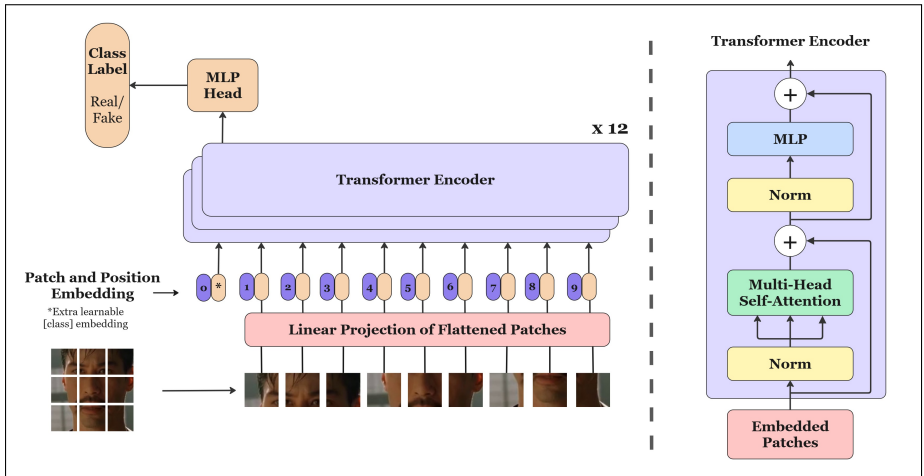
Gambar 3.9 Arsitektur model spasial berbasis Vision Transformer (ViT)
