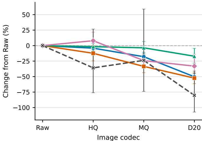
(b) Change from model-specific Raw
