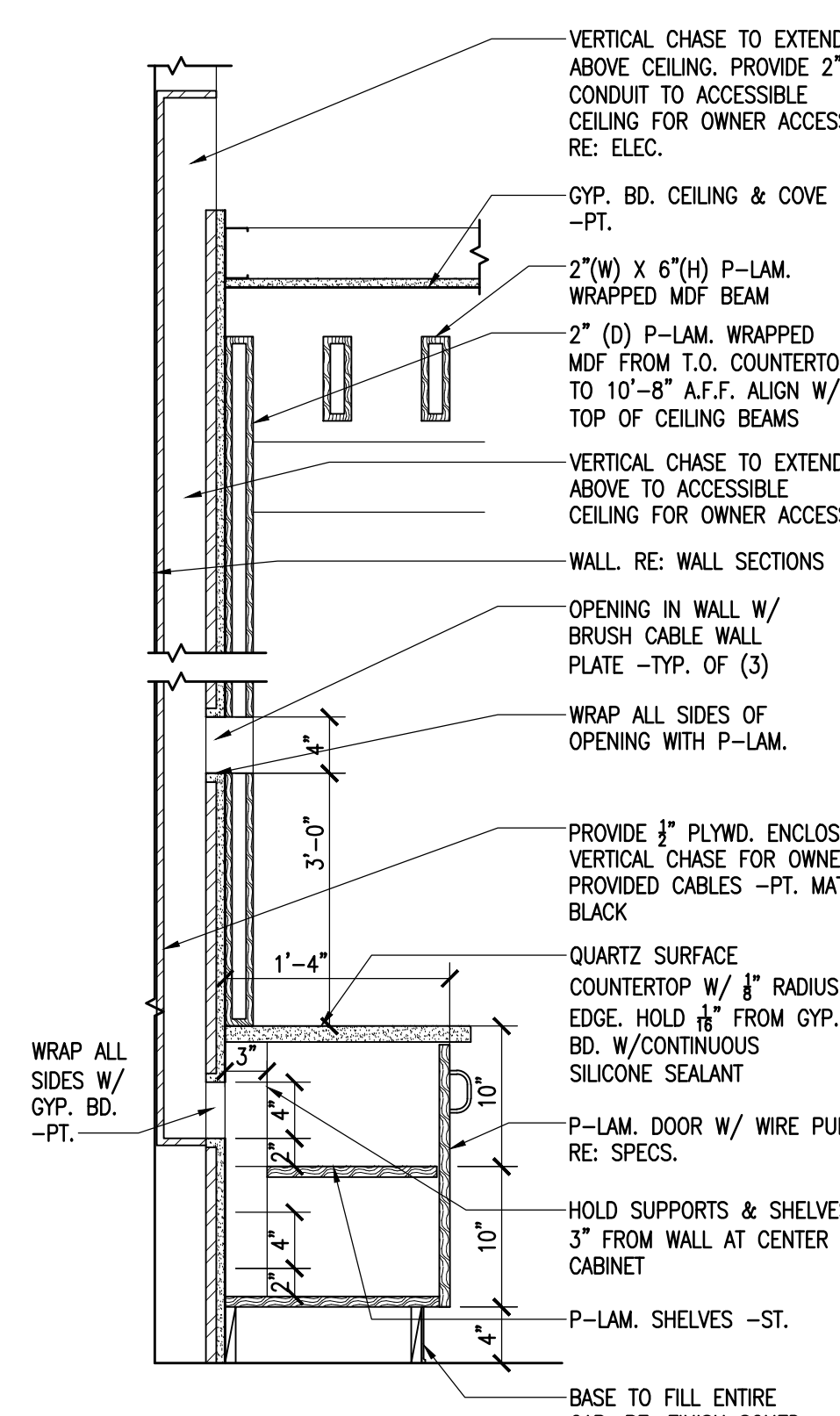
7 SHELVING DETAIL SCALE: 1"=1'-0"
