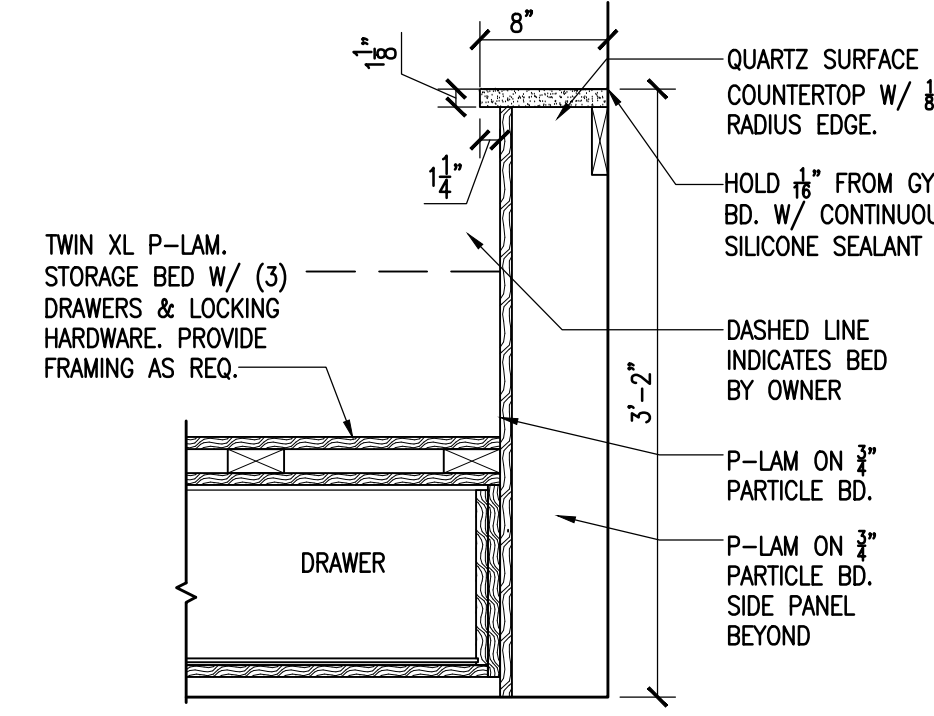
16 HEADBOARD/SHELF DETAIL - BUNK ROOMS SCALE: 1"=1'-0"
