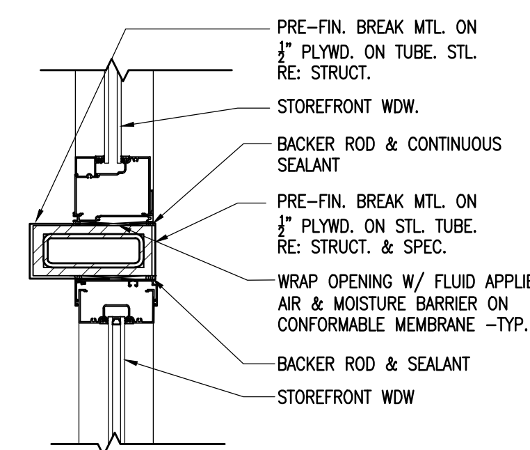
12 HEAD/SILL DETAIL SCALE: 1-1/2" = 1'-0"
