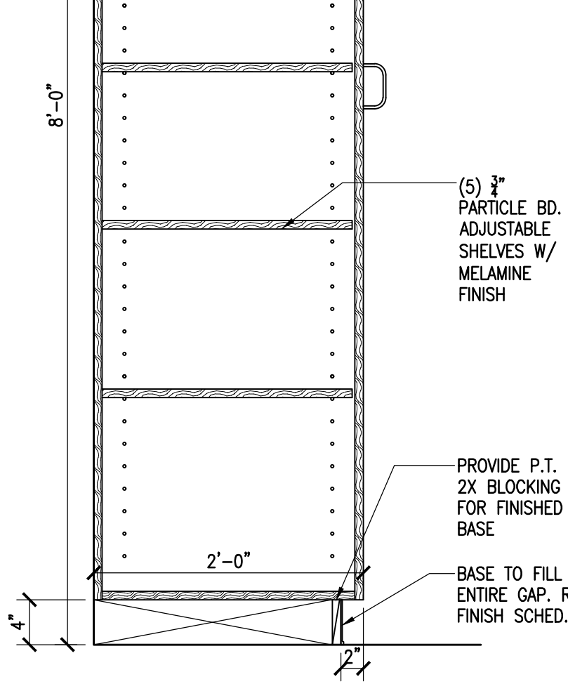
5 CASEWORK DETAIL - LAUNDRY SCALE: 1"=1'-0"
