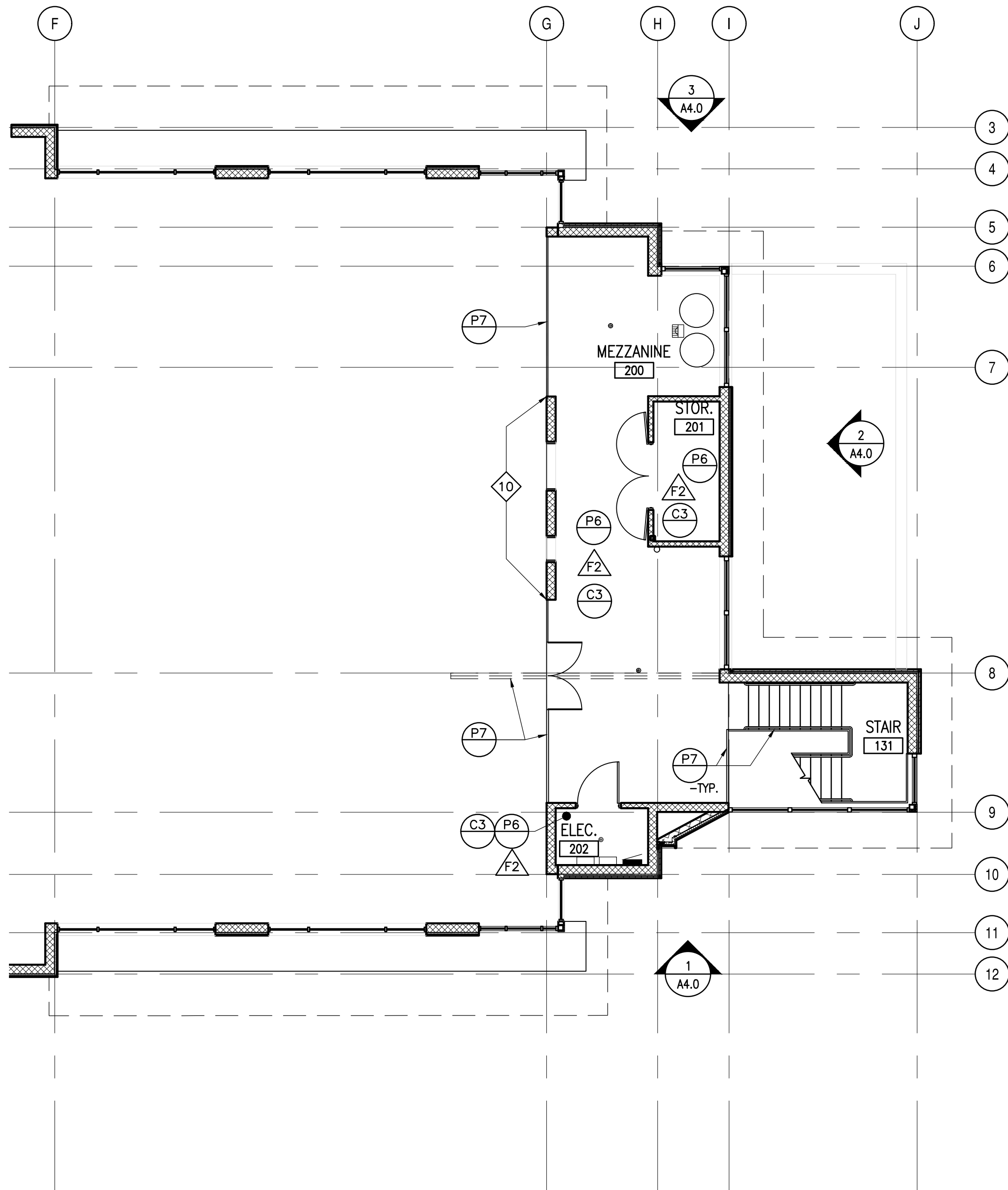
1 MEZZANINE FINISH PLAN SCALE: 1/8"=1'-0"
