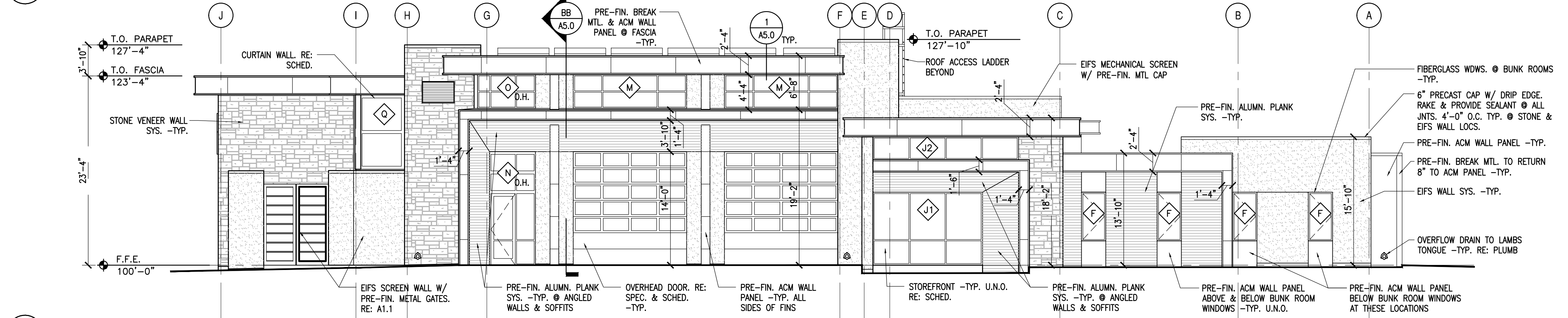
3 NORTH ELEVATION 1/8" = 1'-0"
