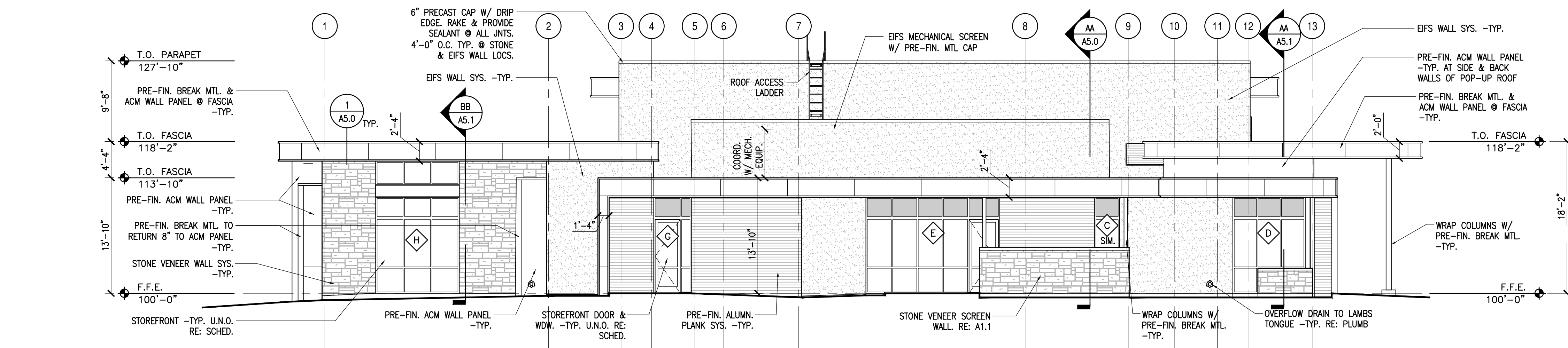
4 WEST ELEVATION 1/8" = 1'-0"
