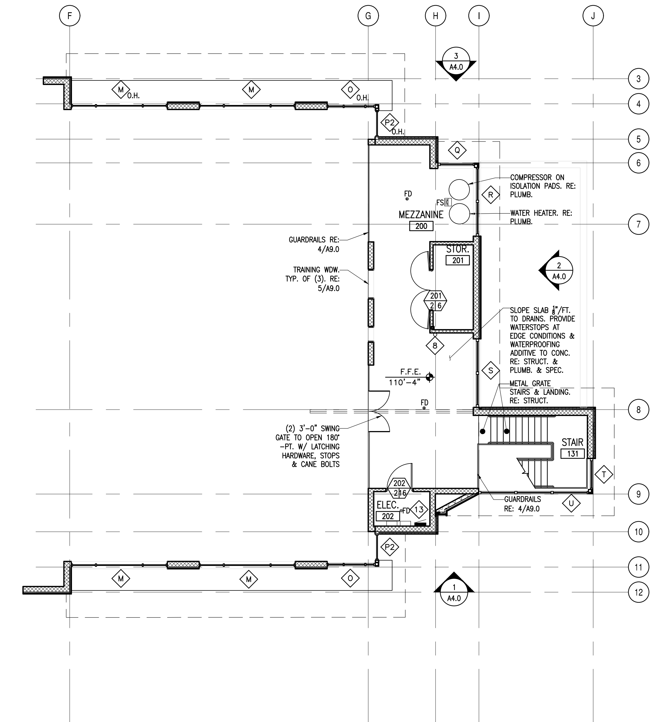
1 MEZZANINE FLOOR PLAN SCALE: 1/8"=1'-0"
