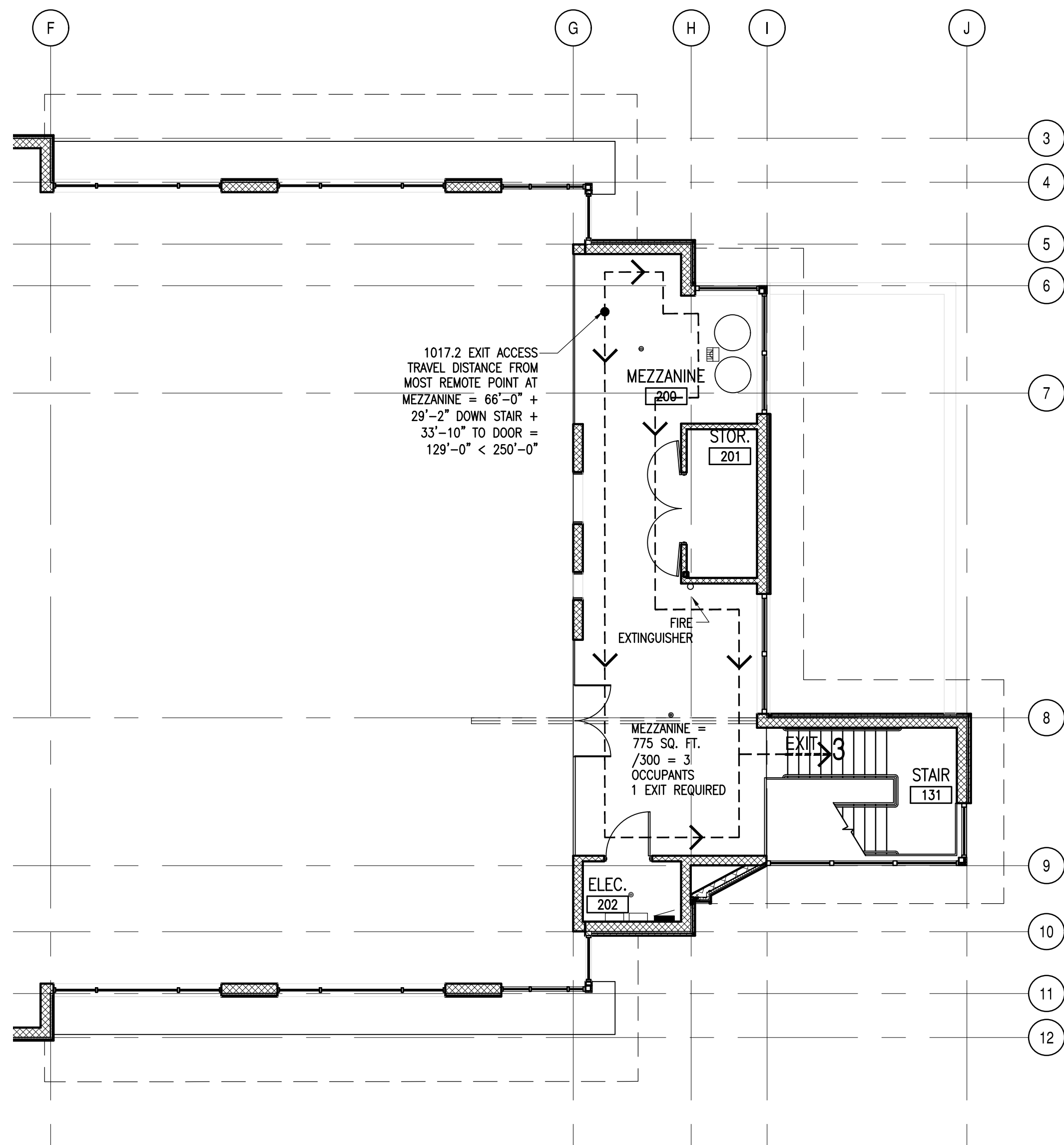
1 MEZZANINE CODE PLAN SCALE: 1/8"=1'-0"
