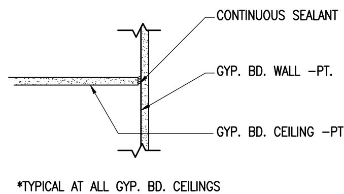
4 TYPICAL GYP. BD. CEILING DETAIL SCALE: 1-1/2"=1'-0"
