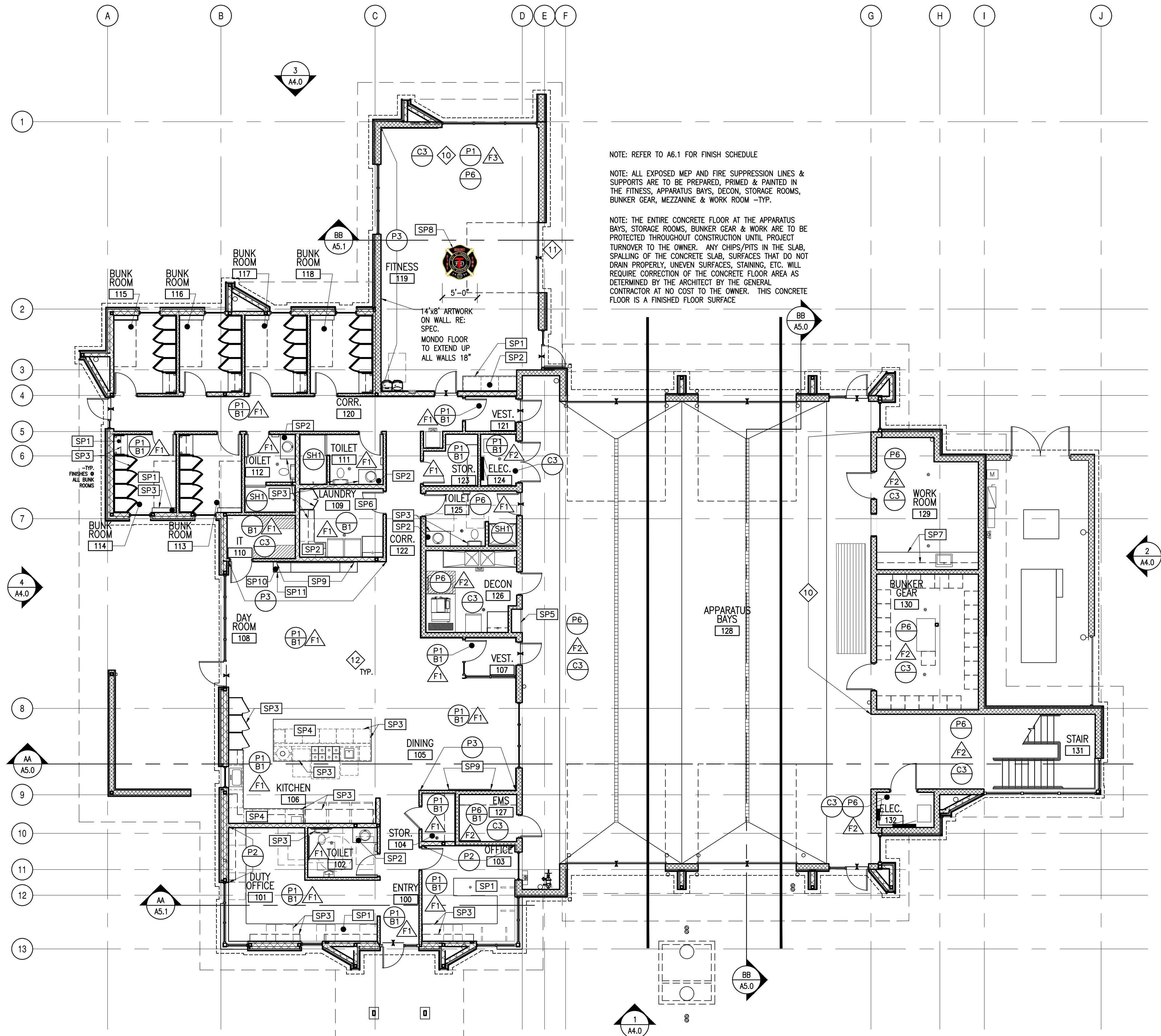
1 MAIN LEVEL FINISH PLAN SCALE: 1/8"=1'-0"
