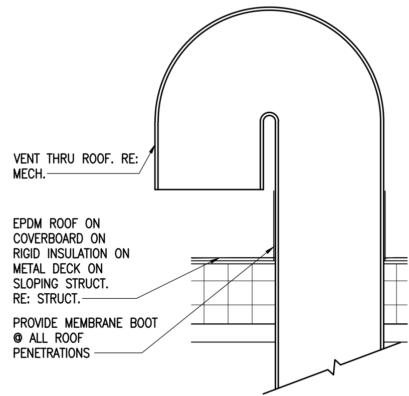
2 VENT THUR EPDM ROOF DETAIL SCALE: 1-1/2"=1'-0"
