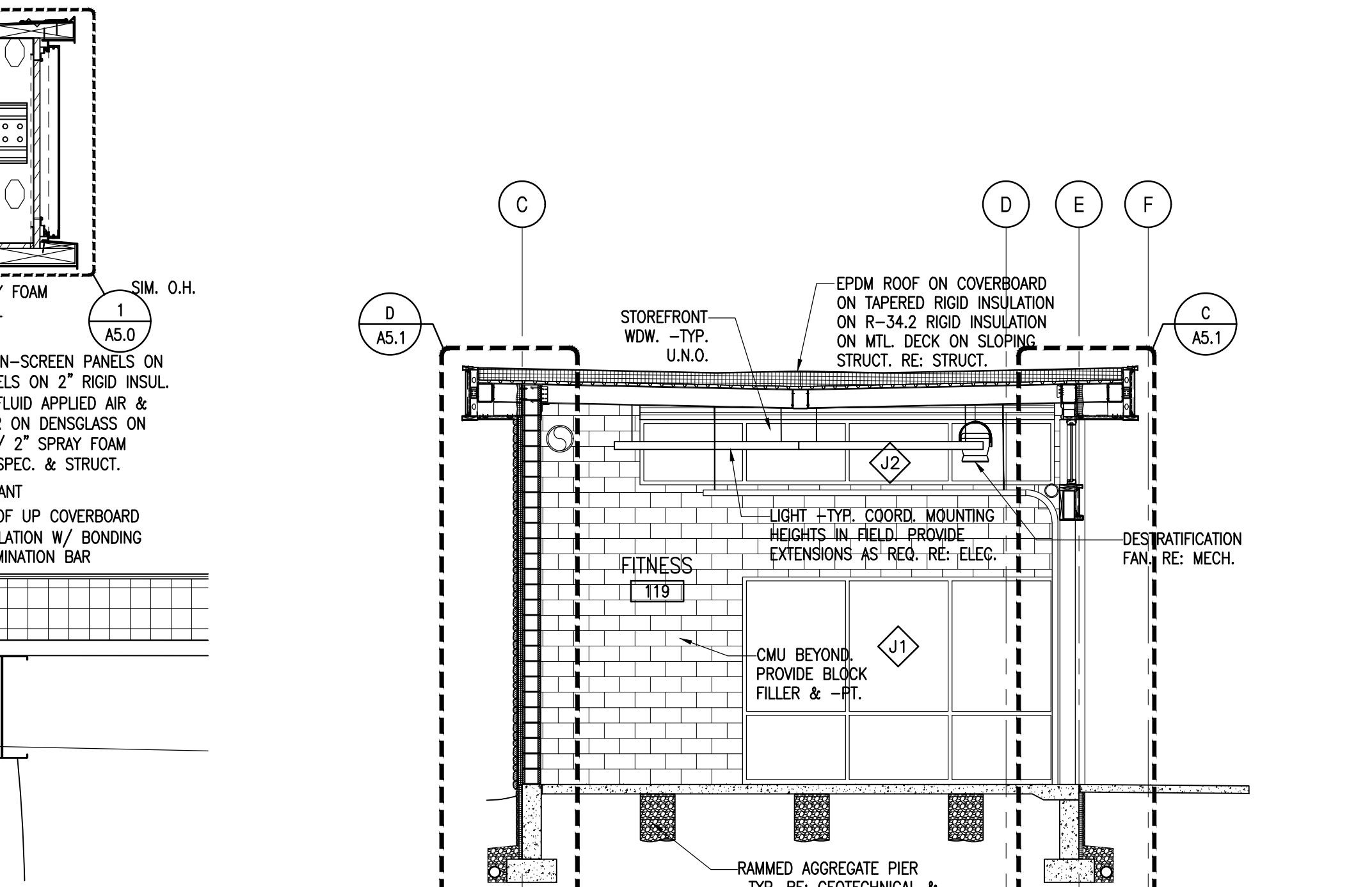
BB WALL SECTION SCALE: 3/16"=1'-0"
