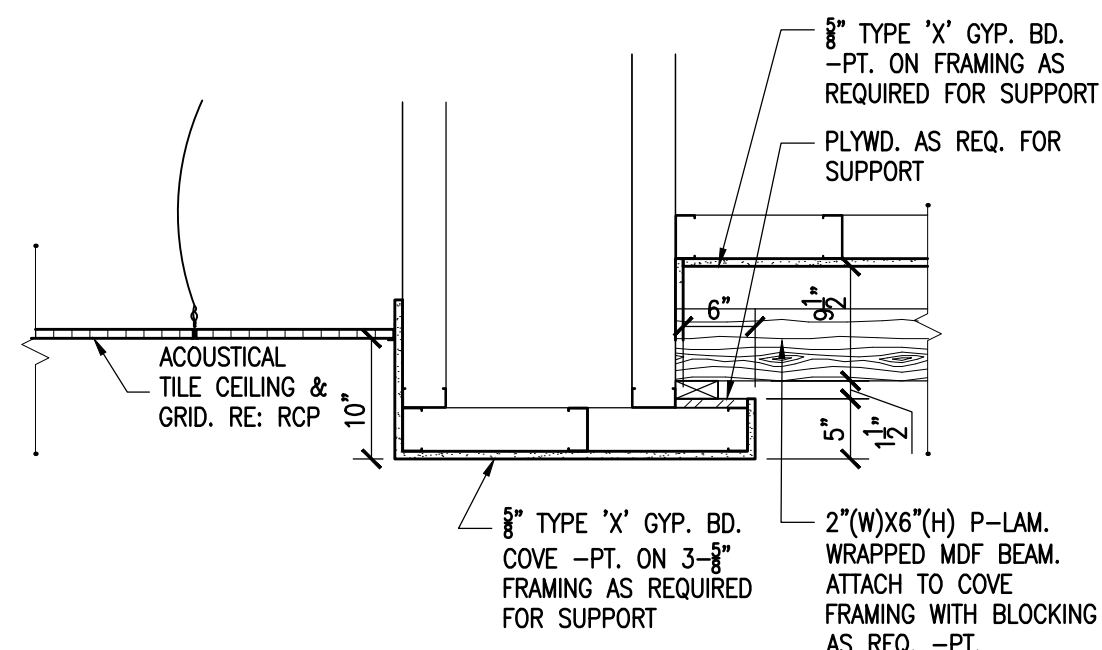
5 COVE CEILING & P-LAM. BEAM DETAIL SCALE: 3/4"=1'-0"
