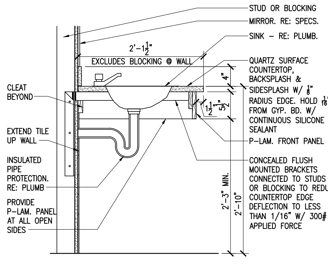
11 CASEWORK DETAIL @ ADA TOILET ROOMS SCALE: 1"=1'-0"
