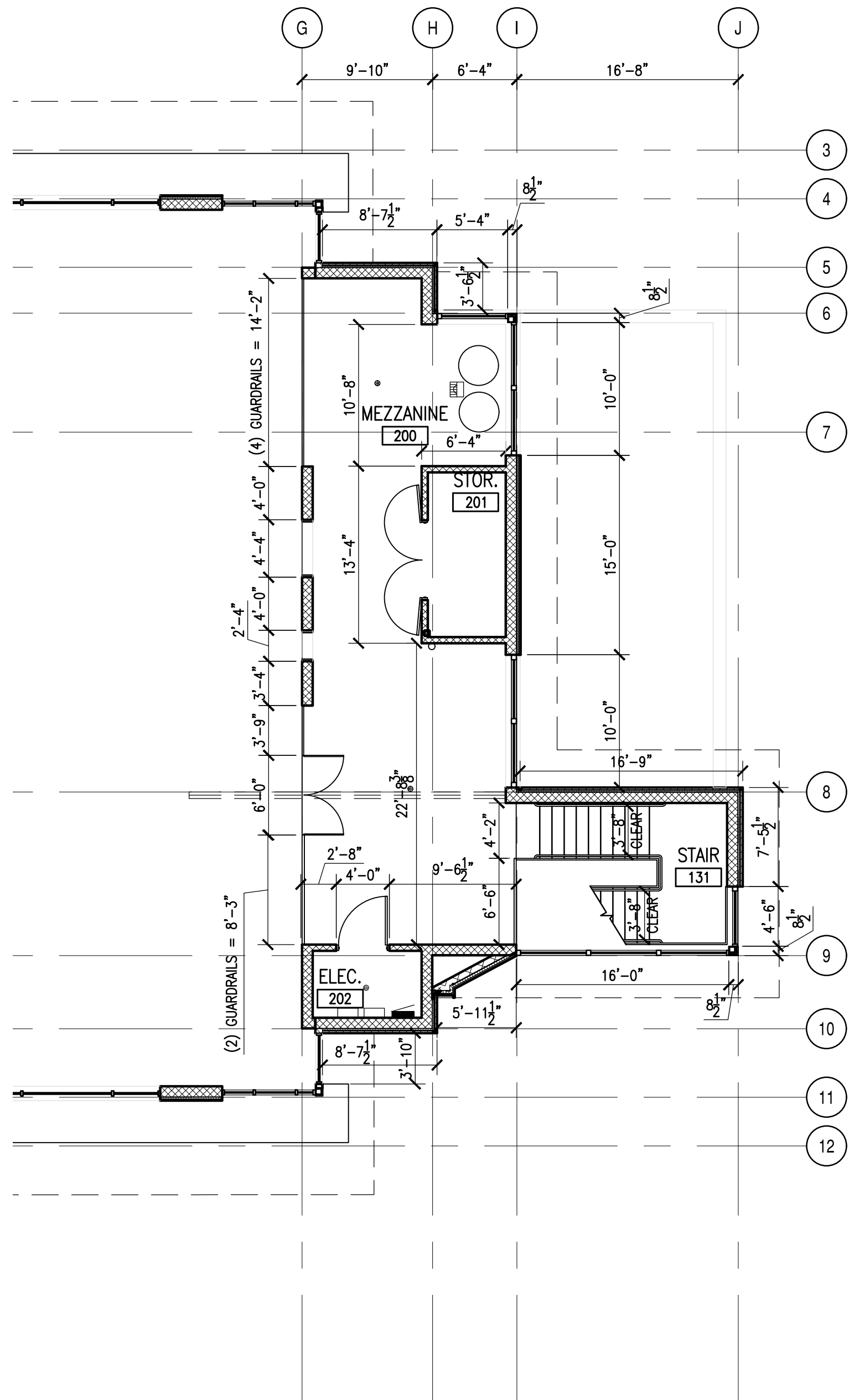
1 MEZZANINE DIMENSION PLAN SCALE: 1/8"=1'-0"
