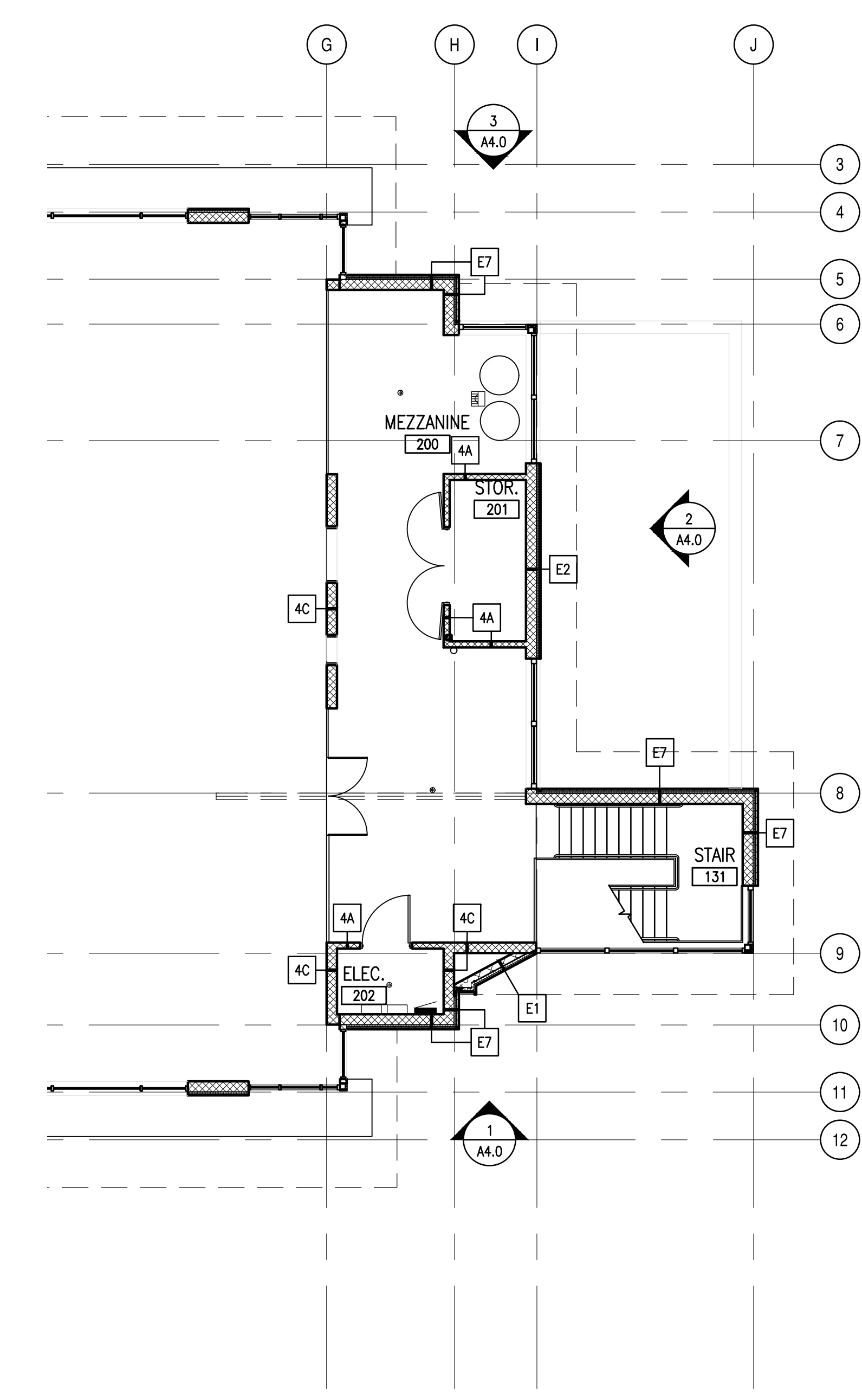
1 MEZZANINE WALL TYPE PLAN SCALE: 1/8"=1'-0"
