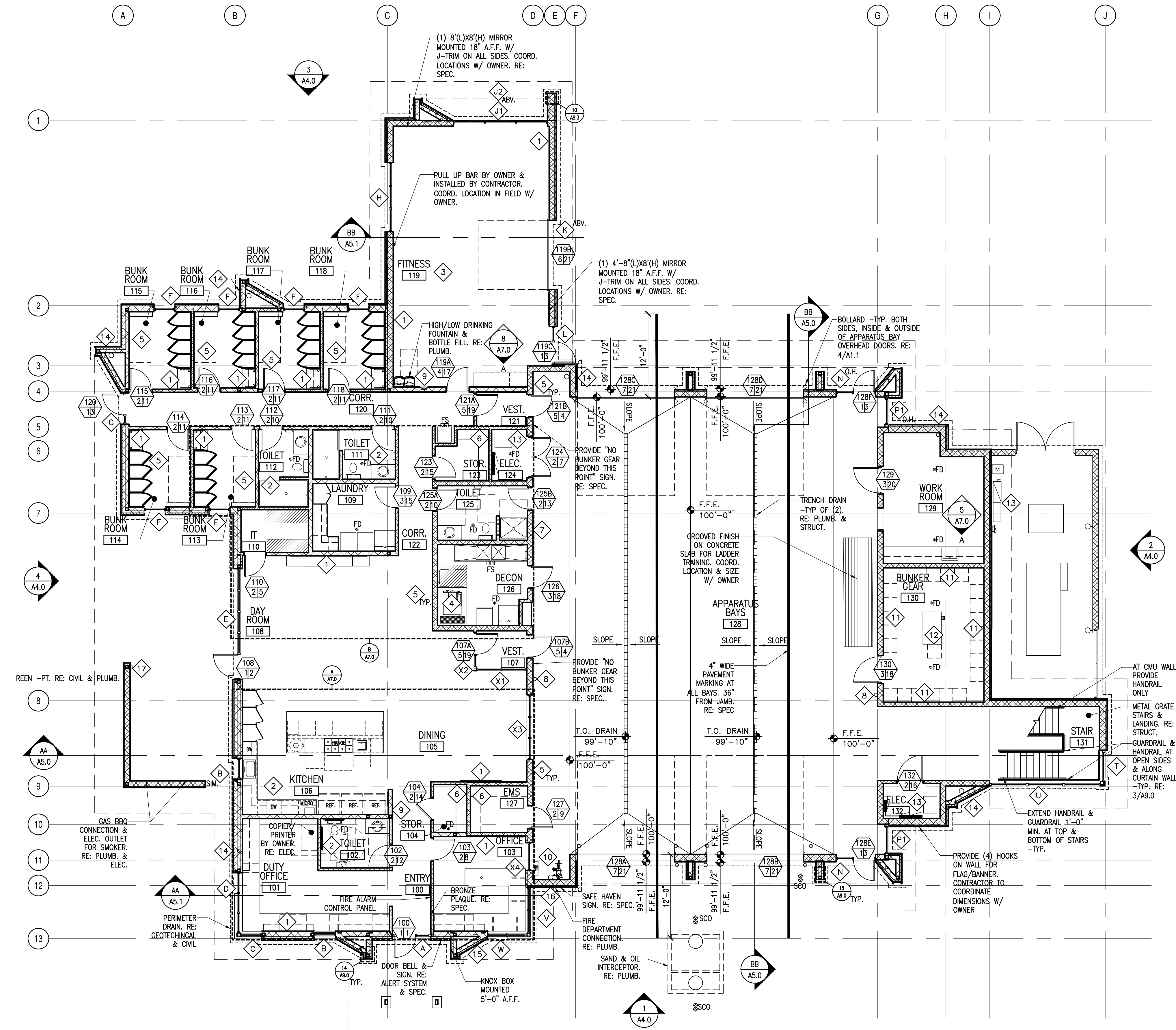
1 MAIN LEVEL FLOOR PLAN SCALE: 1/8"=1'-0"
