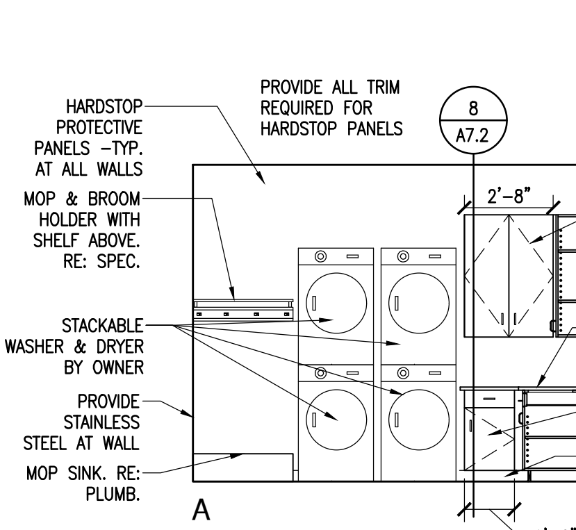
3 INTERIOR ELEVATION - LAUNDRY 109 SCALE: 1/4"=1'-0"
