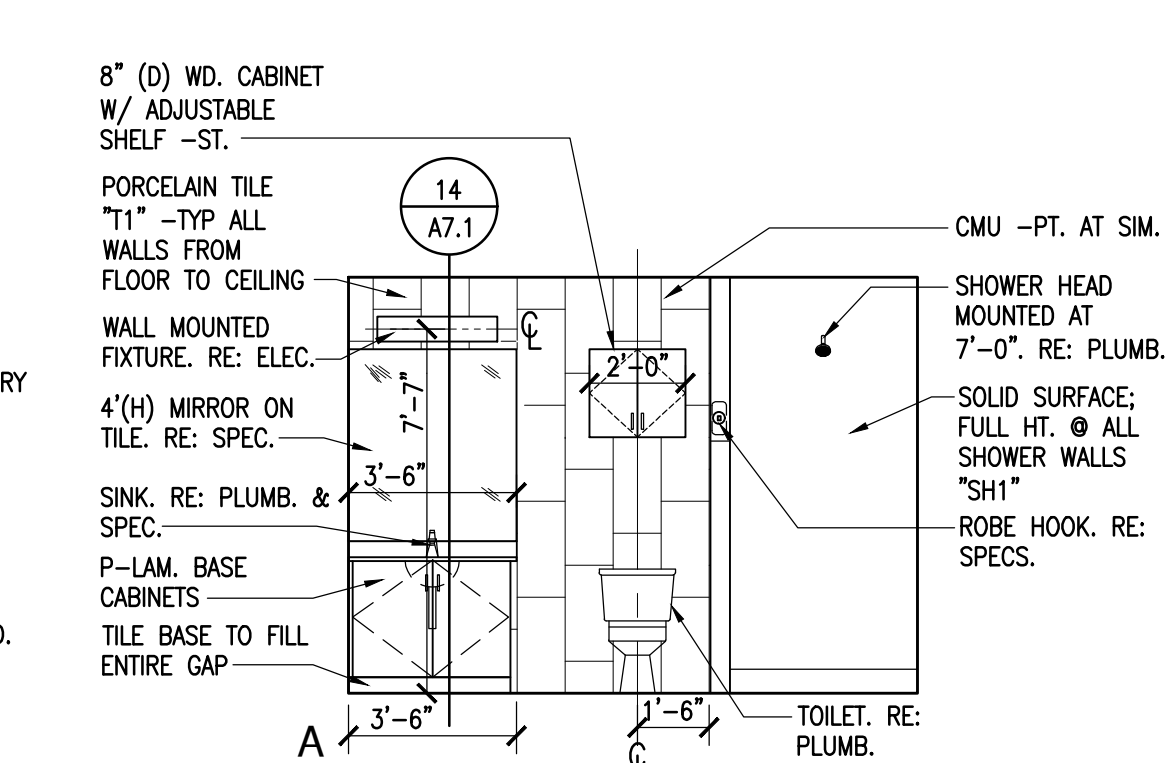
2 INTERIOR ELEVATION - TOILET ROOM 111 & 112 (O.H. & SIM. @ 125) SCALE: 1/4"=1'-0"
