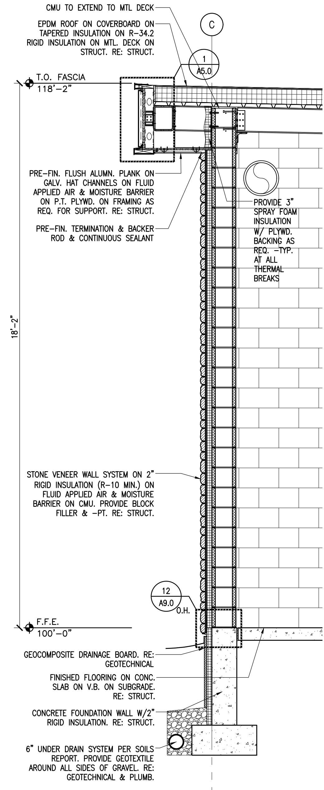
D BUILDING SECTION SCALE: 1/2"=1'-0"
