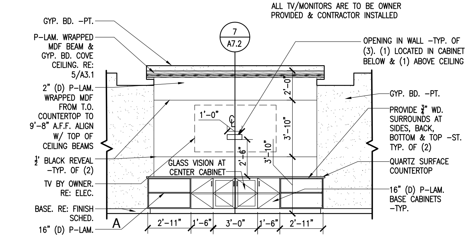
1 INTERIOR ELEVATION - DAY ROOM 108 SCALE: 1/4"=1'-0"
