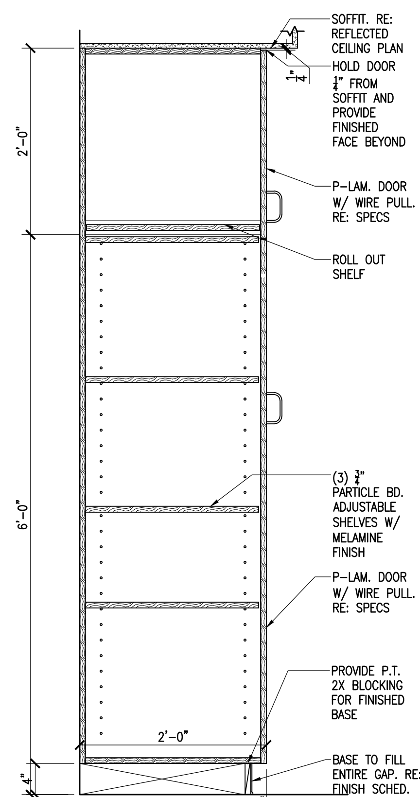
4 CASEWORK DETAIL - KITCHEN SCALE: 1"=1'-0"
