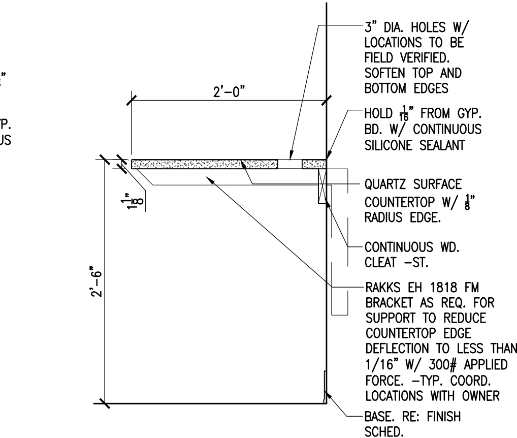
15 DESK DETAIL @ BUNK ROOMS SCALE: 1"=1'-0"
