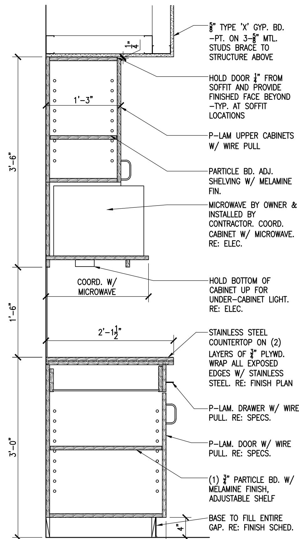
3 CASEWORK DETAIL - KITCHEN SCALE: 1"=1'-0"
