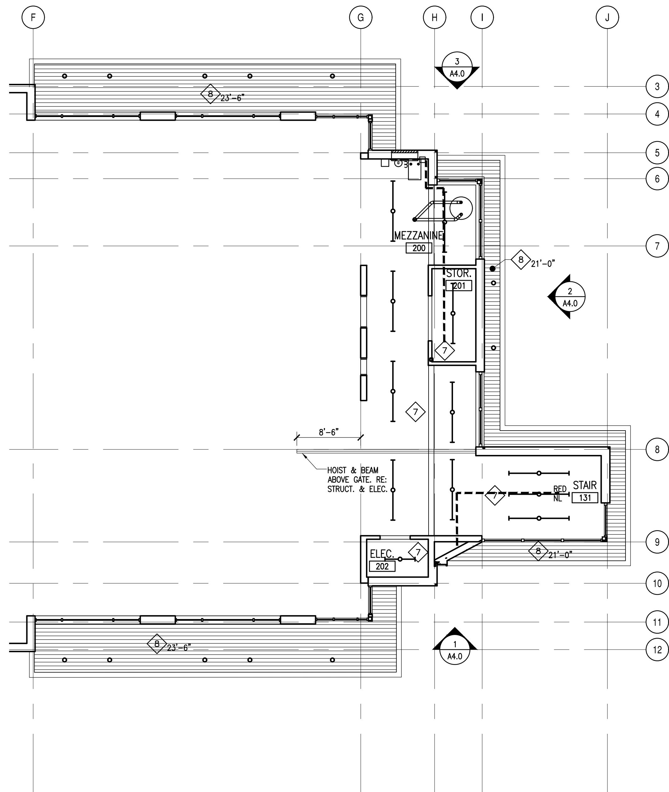
1 MEZZANINE FLOOR PLAN SCALE: 1/8"=1'-0"
