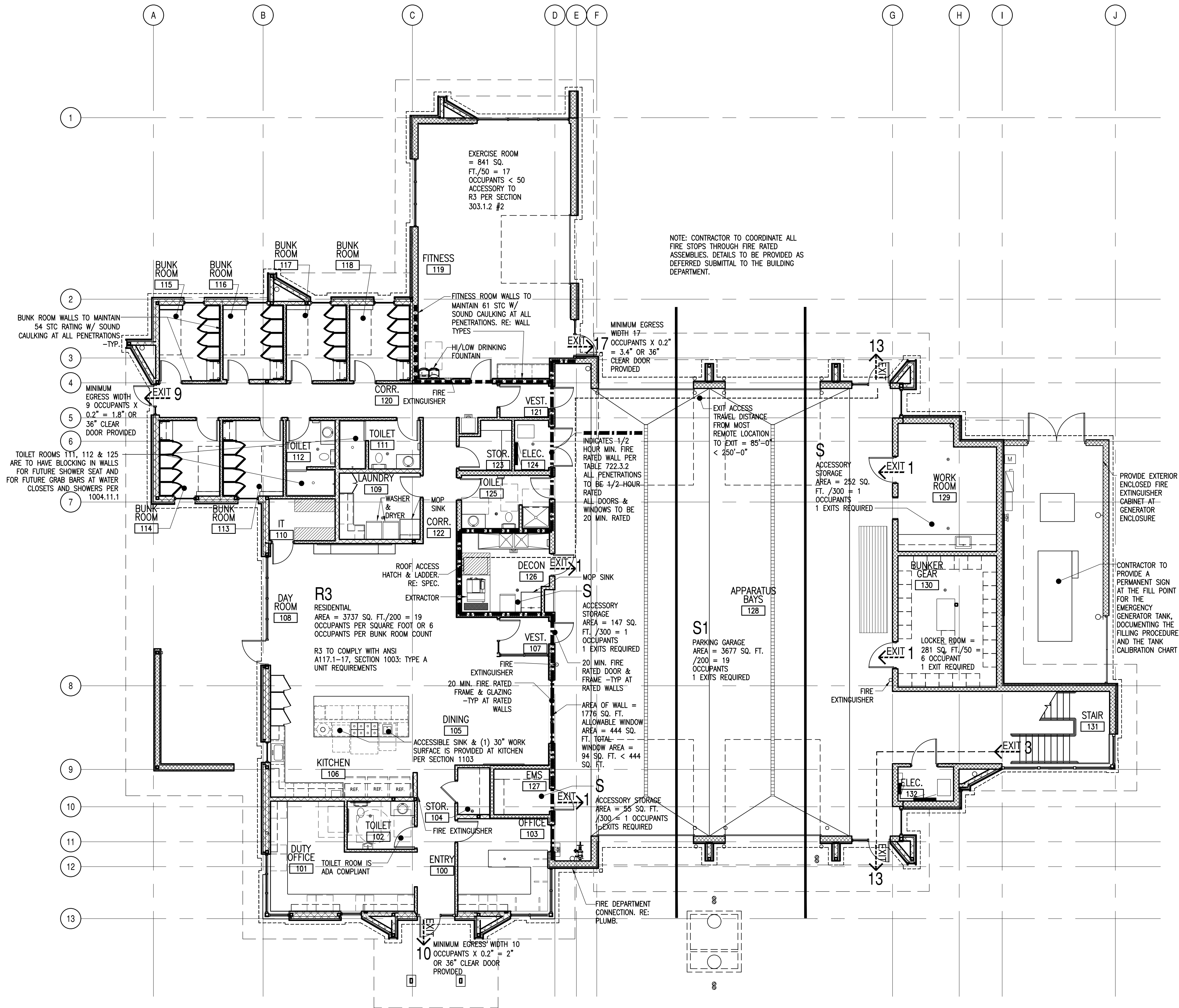
1 MAIN LEVEL CODE PLAN SCALE: 1/8"=1'-0"
