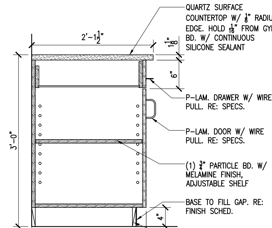
1 CASEWORK DETAIL SCALE: 1"=1'-0"
