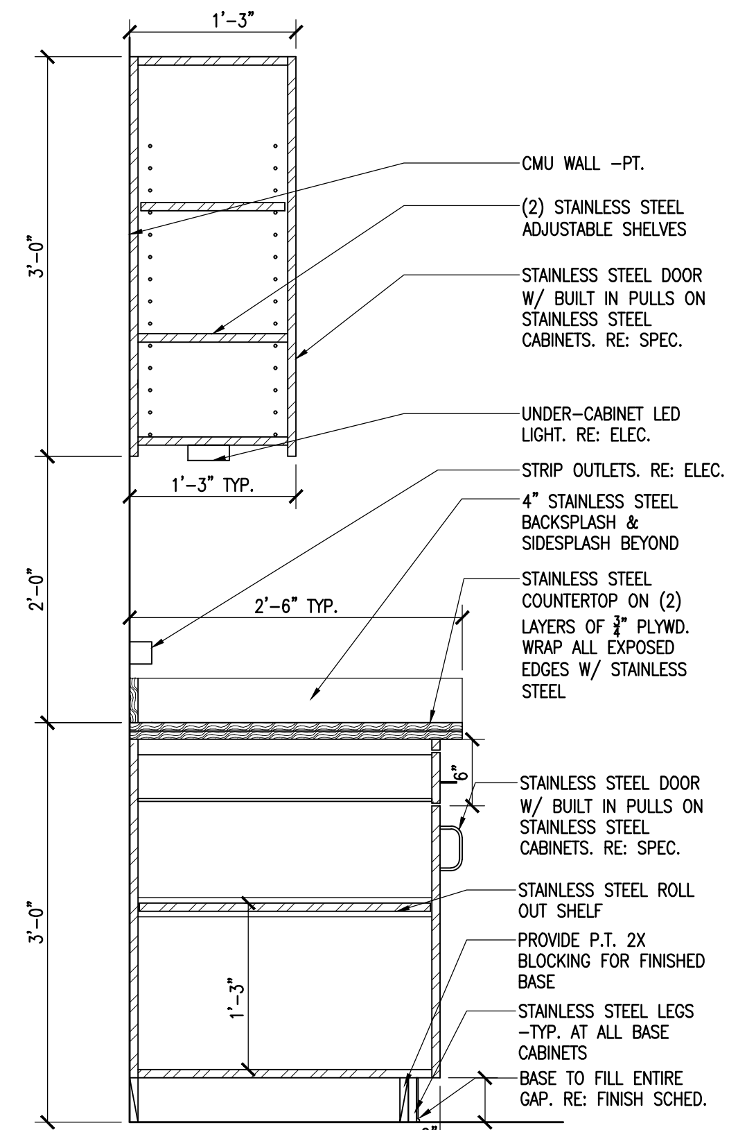
6 CASEWORK DETAIL - WORK ROOM SCALE: 1"=1'-0"
