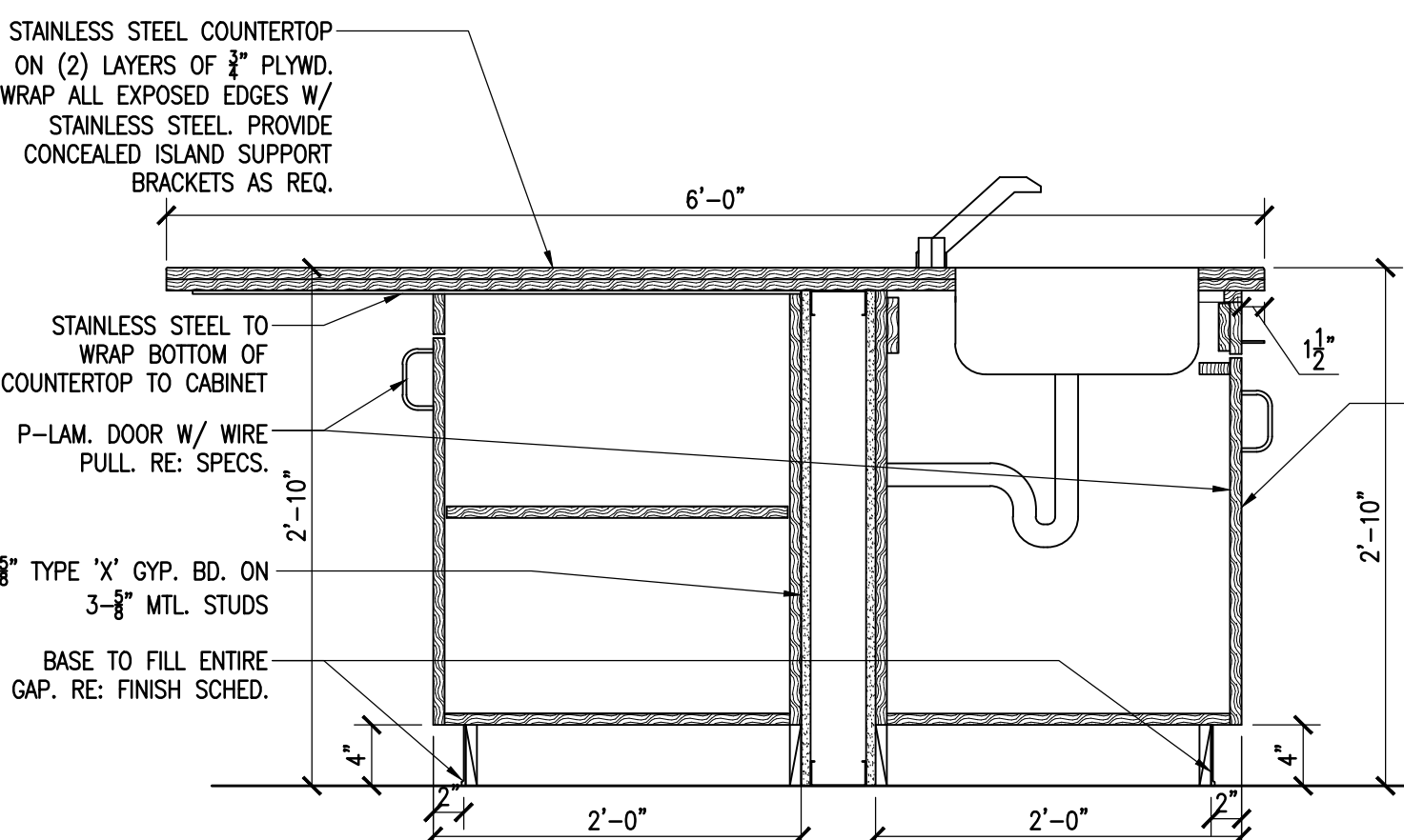
13 CASEWORK DETAIL - KITCHEN SCALE: 1"=1'-0"
