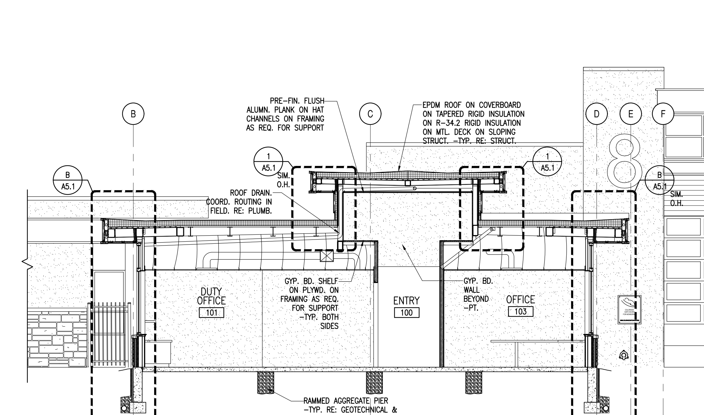
AA WALL SECTION SCALE: 3/16"=1'-0"
