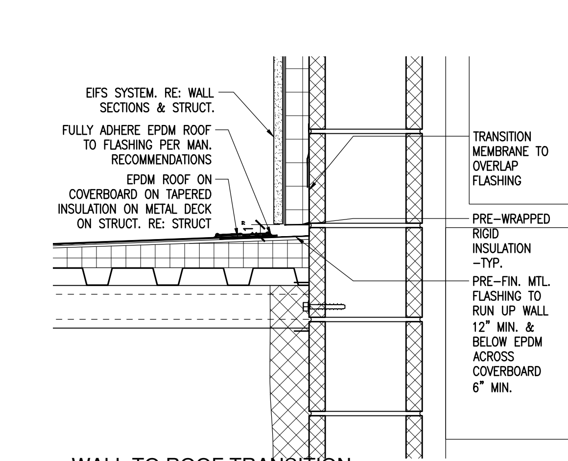
3 WALL TO ROOF TRANSITION AT APPARATUS BAYS (SIM @ ACM.) SCALE: 1/2"=1'-0"
