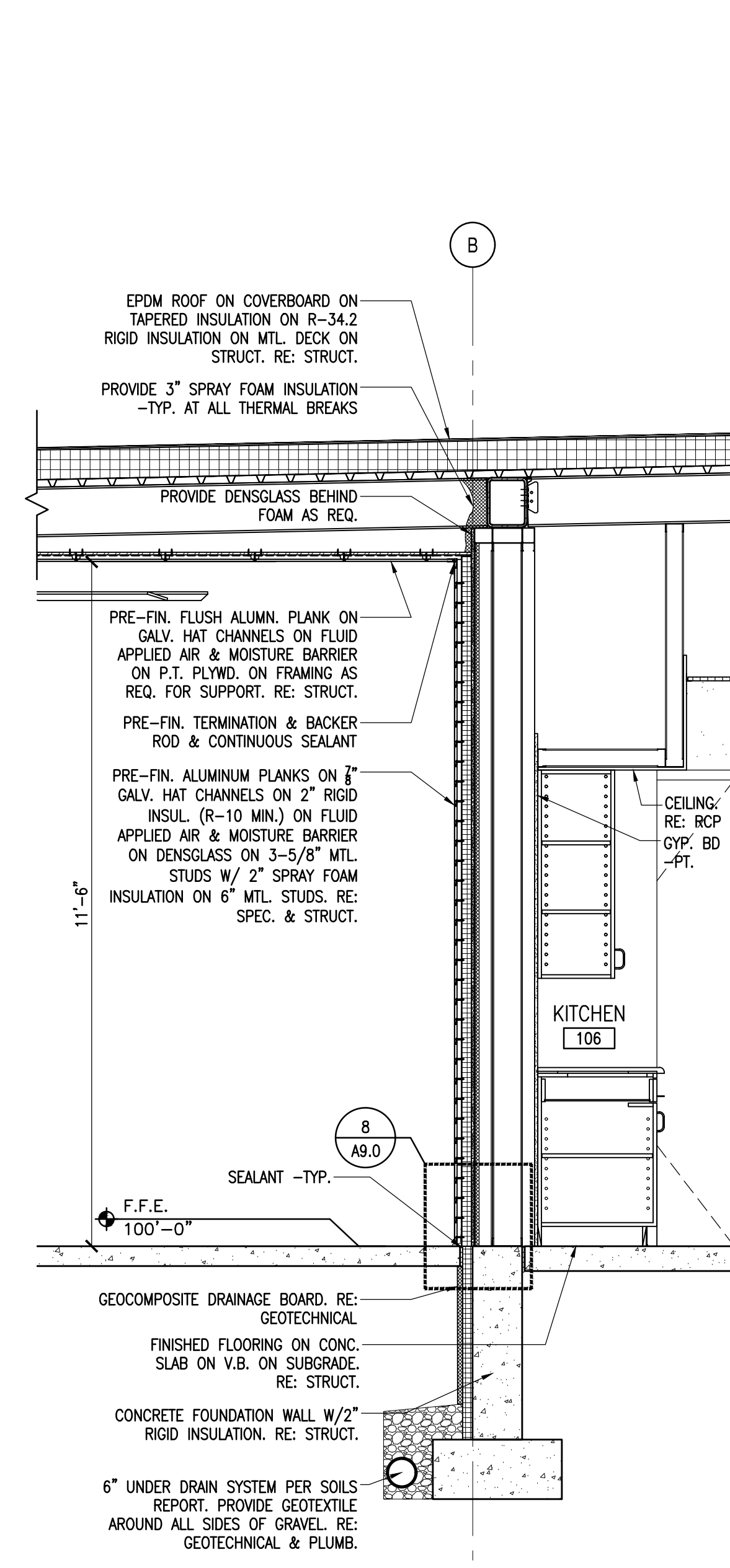
A BUILDING SECTION SCALE: 1/2"=1'-0"
