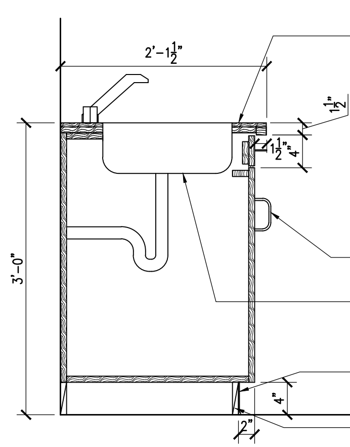
12 CASEWORK DETAIL - KITCHEN SCALE: 1"=1'-0"
