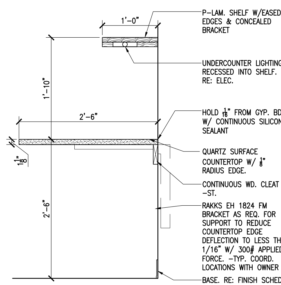
6 DESK DETAIL @ OFFICE SCALE: 1"=1'-0"
