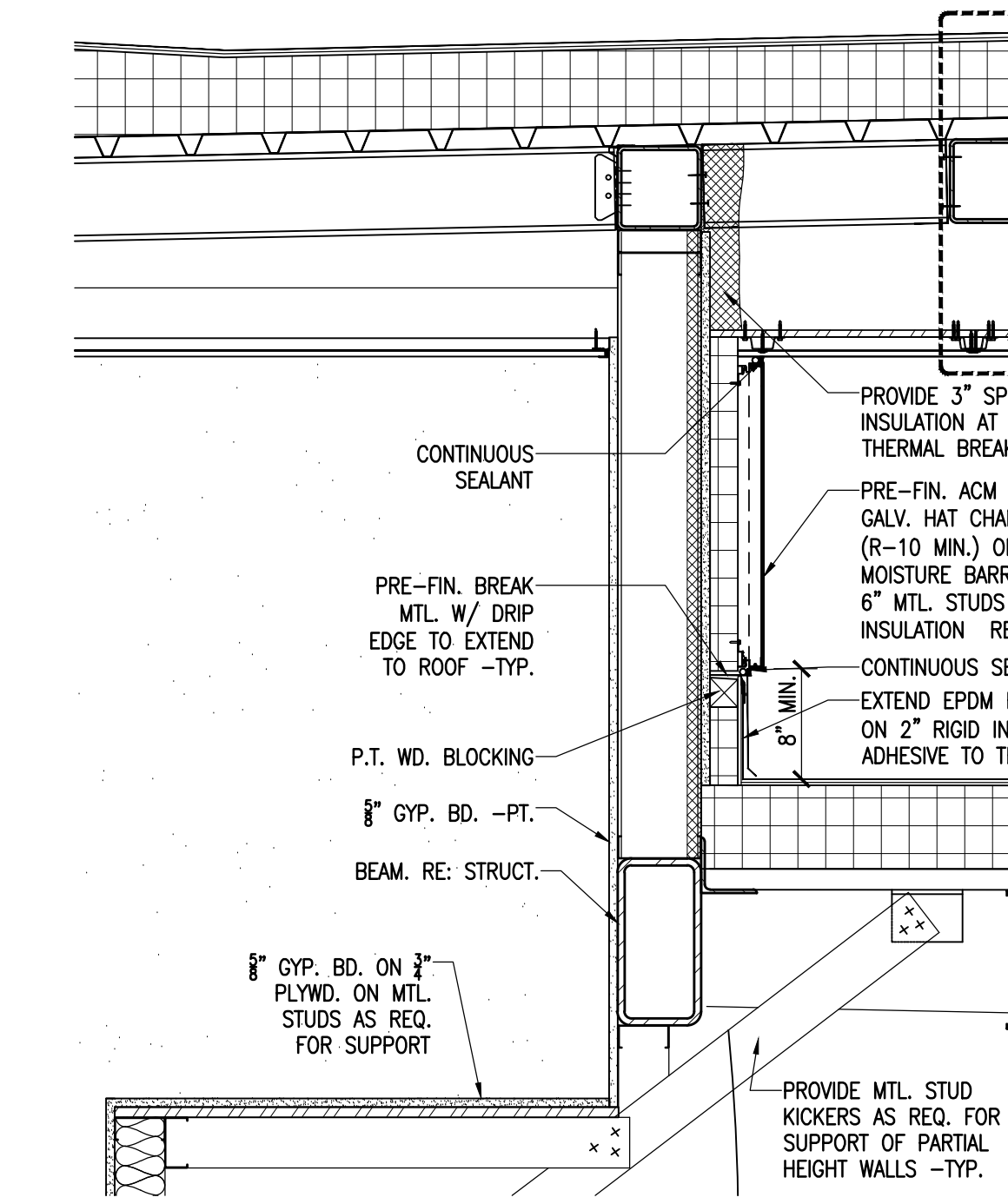
1 WALL TO ROOF AT POP-UP DETAIL SCALE: 1/2"=1'-0"
