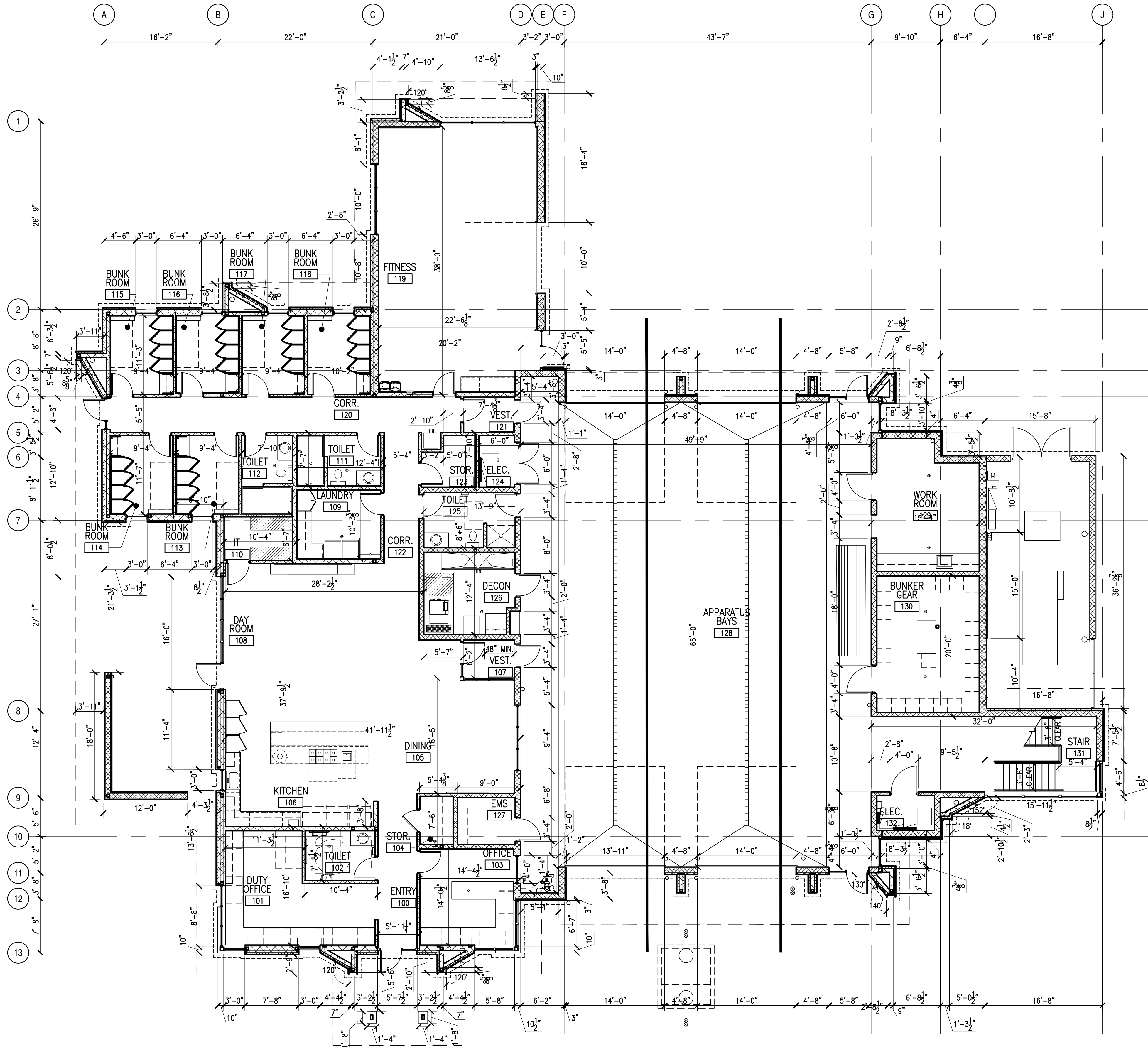
1 MAIN LEVEL DIMENSION PLAN SCALE: 1/8"=1'-0"
