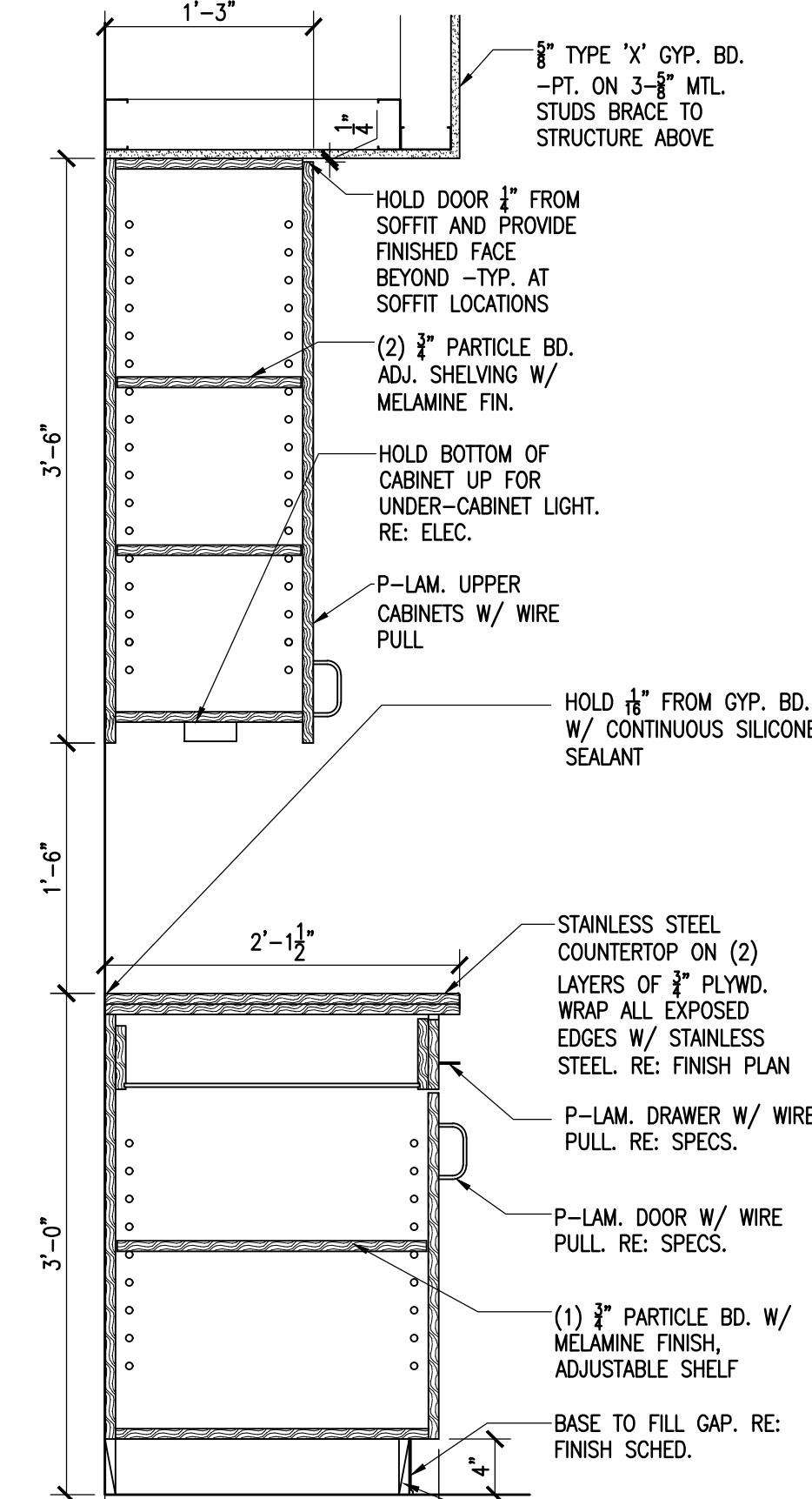
2 CASEWORK DETAIL - KITCHEN SCALE: 1"=1'-0"
