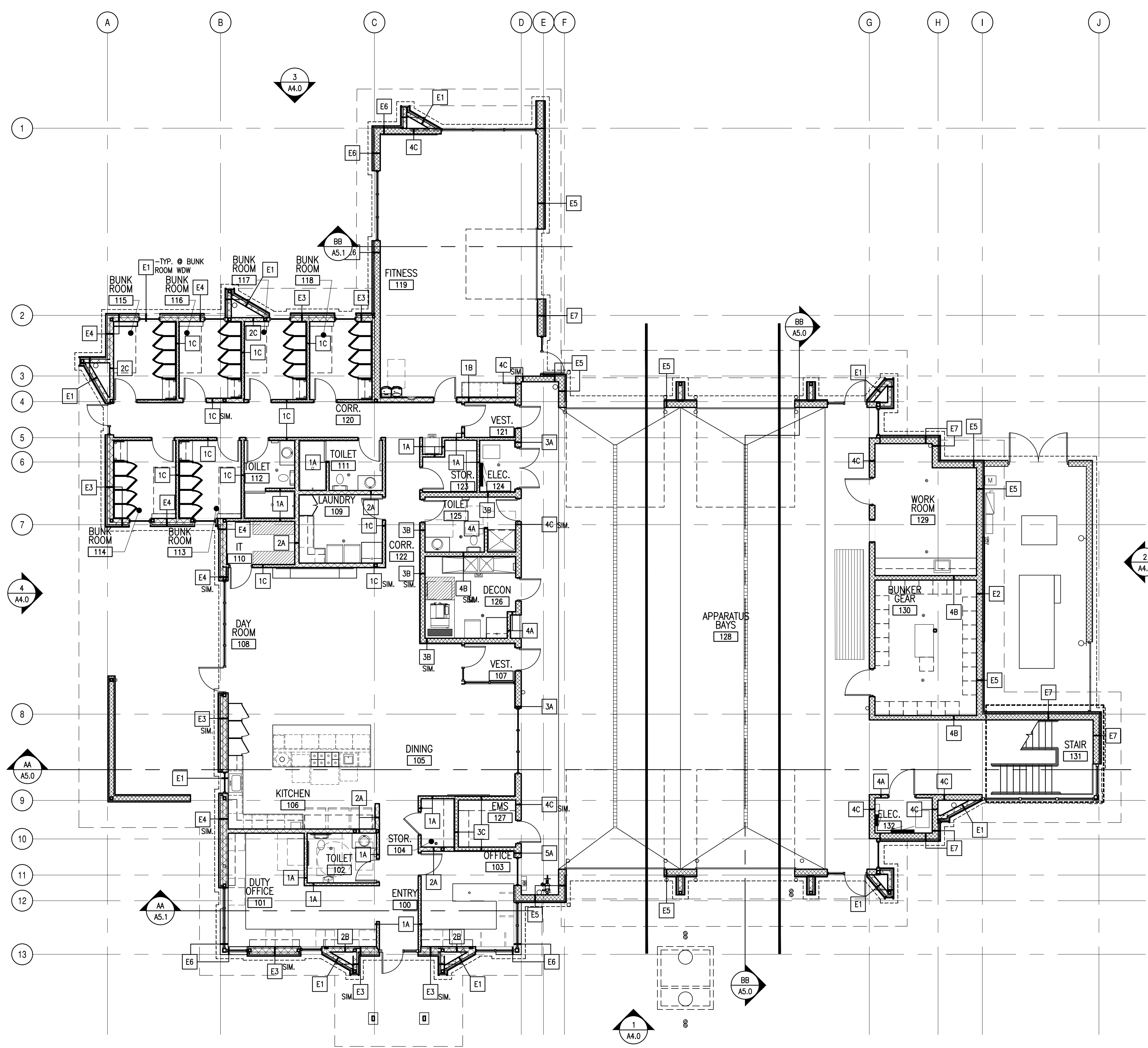
1 MAIN LEVEL WALL TYPE PLAN SCALE: 1/8"=1'-0"
