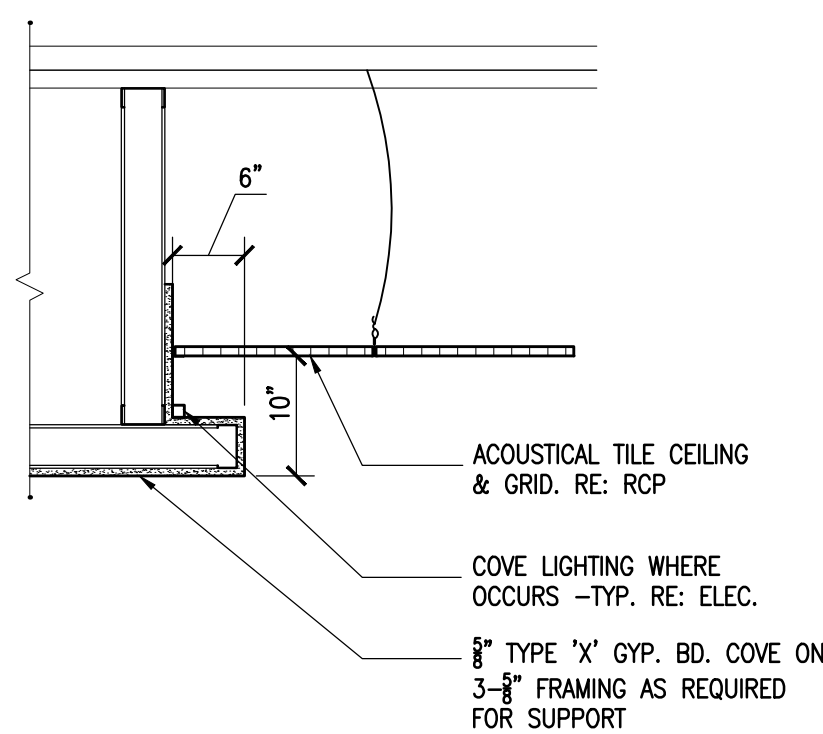
2 COVE CEILING DETAIL SCALE: 3/4"=1'-0"
