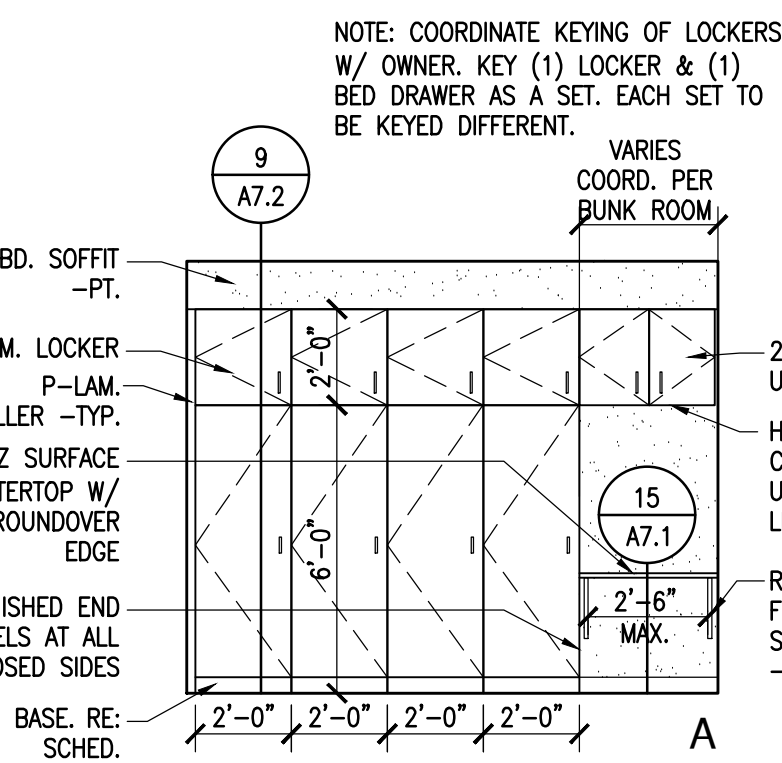
4 INTERIOR ELEVATIONS - BUNK ROOMS SCALE: 1/4"=1'-0"
