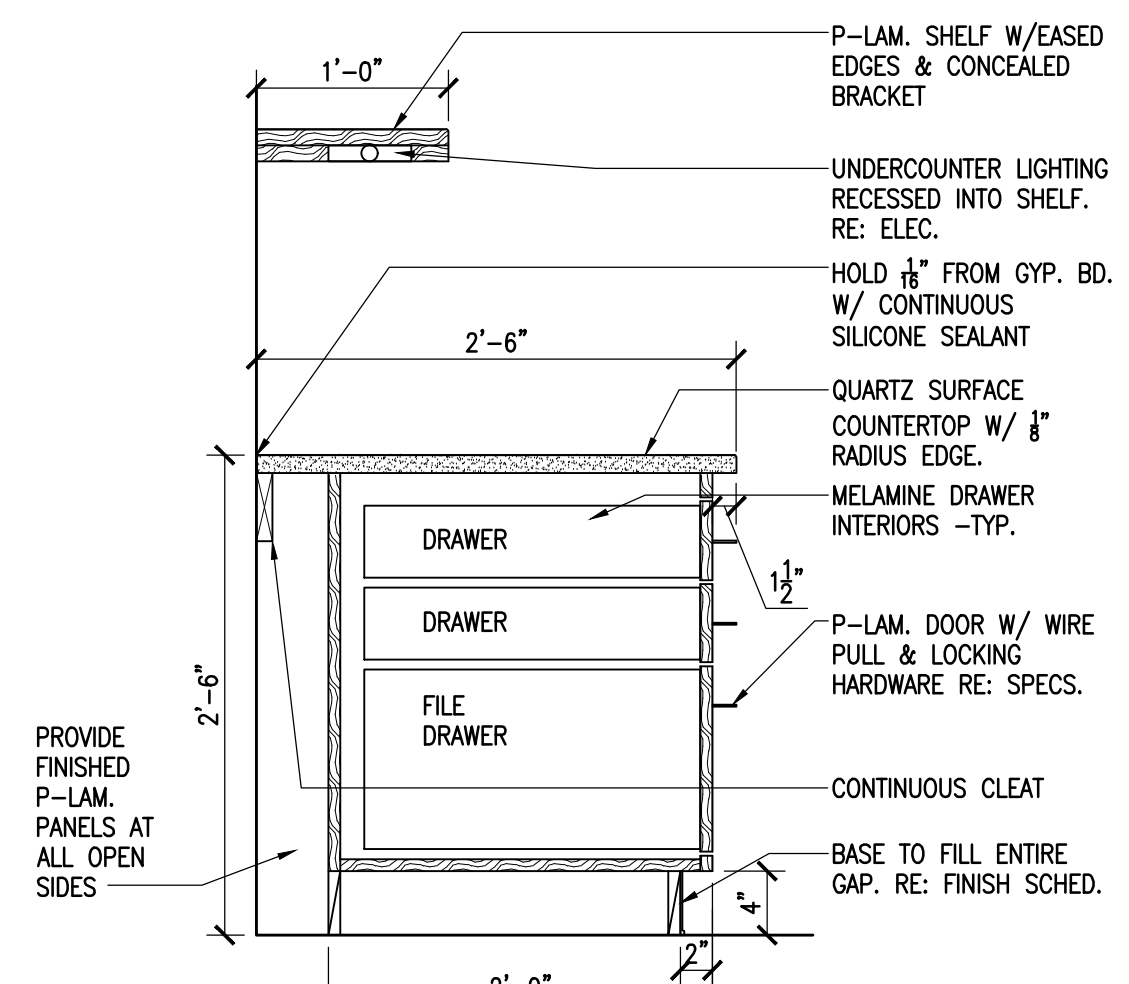
9 CASEWORK DETAIL - OFFICE SCALE: 1"=1'-0"
