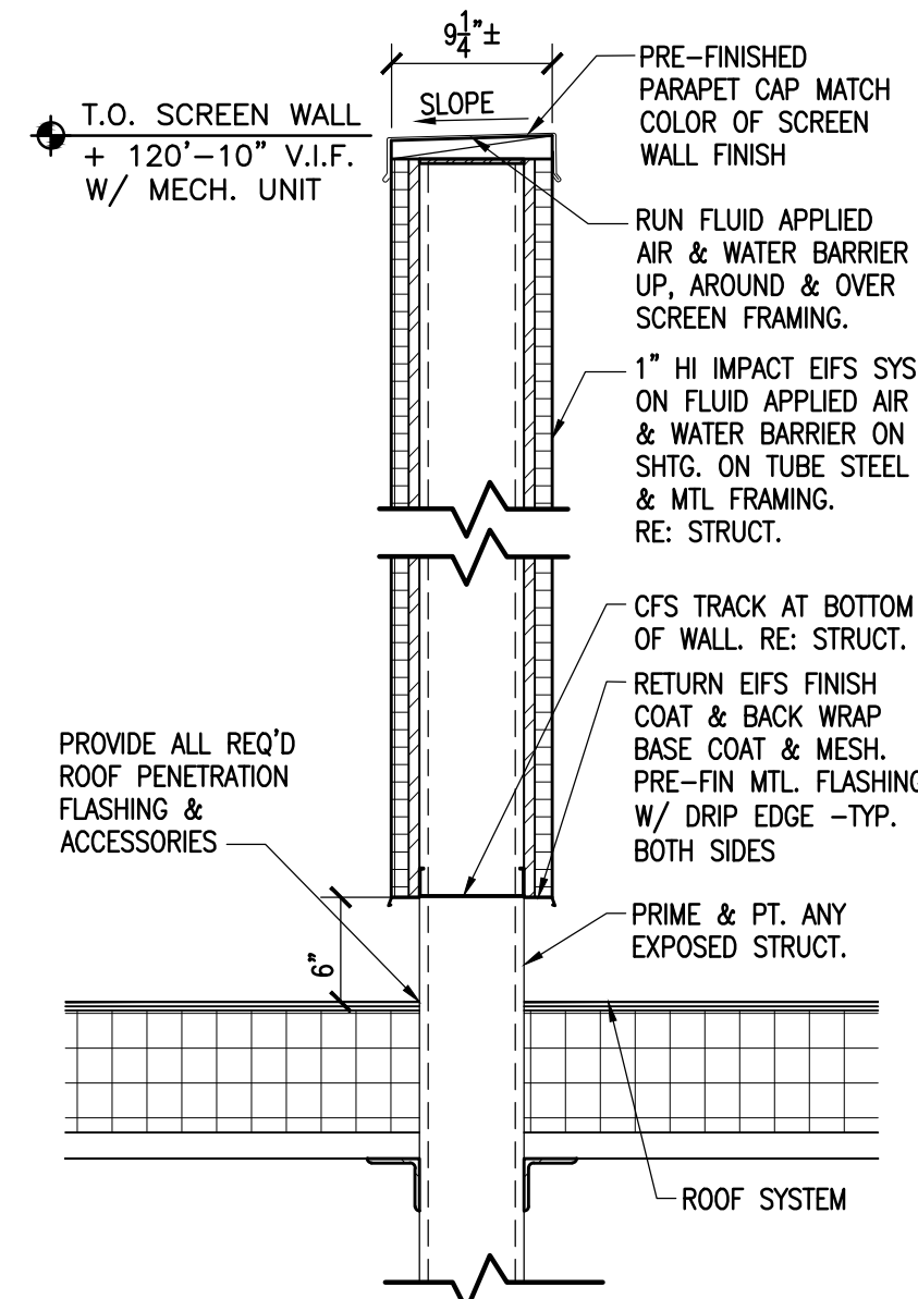
3 MECHANICAL SCREEN SECTION 1"=1'-0"
