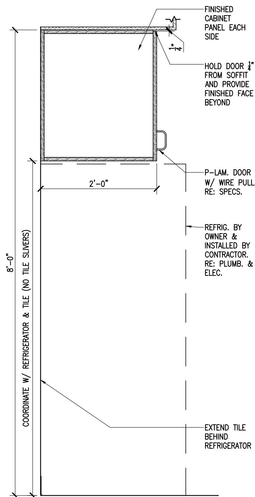
5 CASEWORK DETAIL - KITCHEN SCALE: 1"=1'-0"
