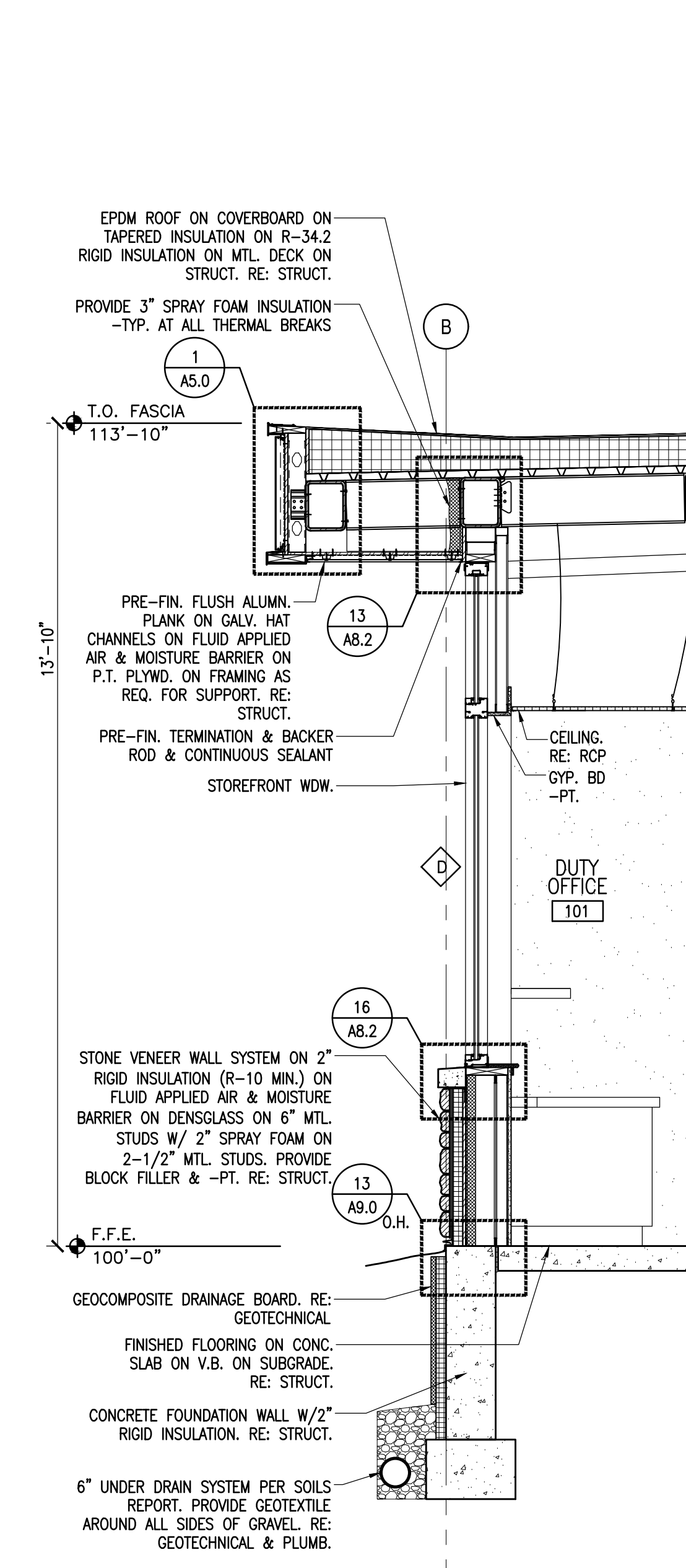
B BUILDING SECTION SCALE: 1/2"=1'-0"
