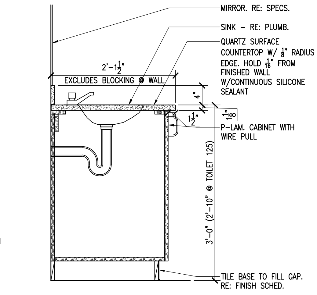
14 CASEWORK DETAIL @ TOILET ROOMS SCALE: 1"=1'-0"
