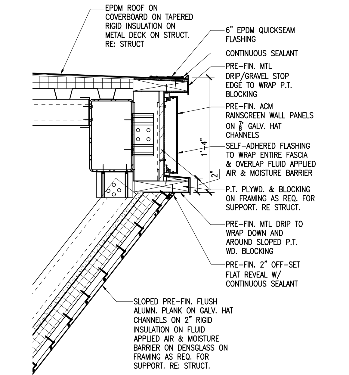
2 FASCIA TO ANGLED WALL DETAIL SCALE: 1/2"=1'-0"
