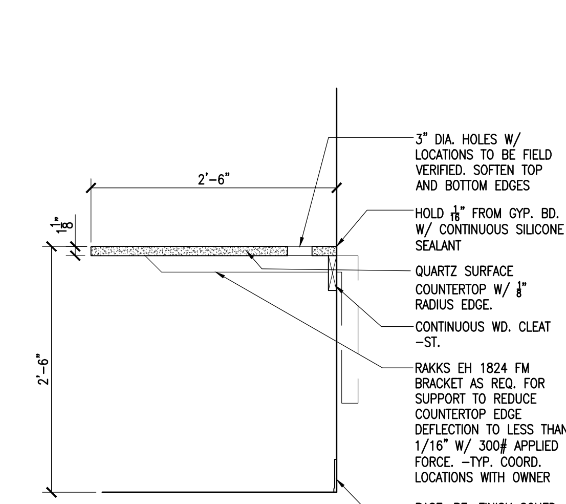
7 DESK DETAIL @ OFFICE SCALE: 1"=1'-0"
