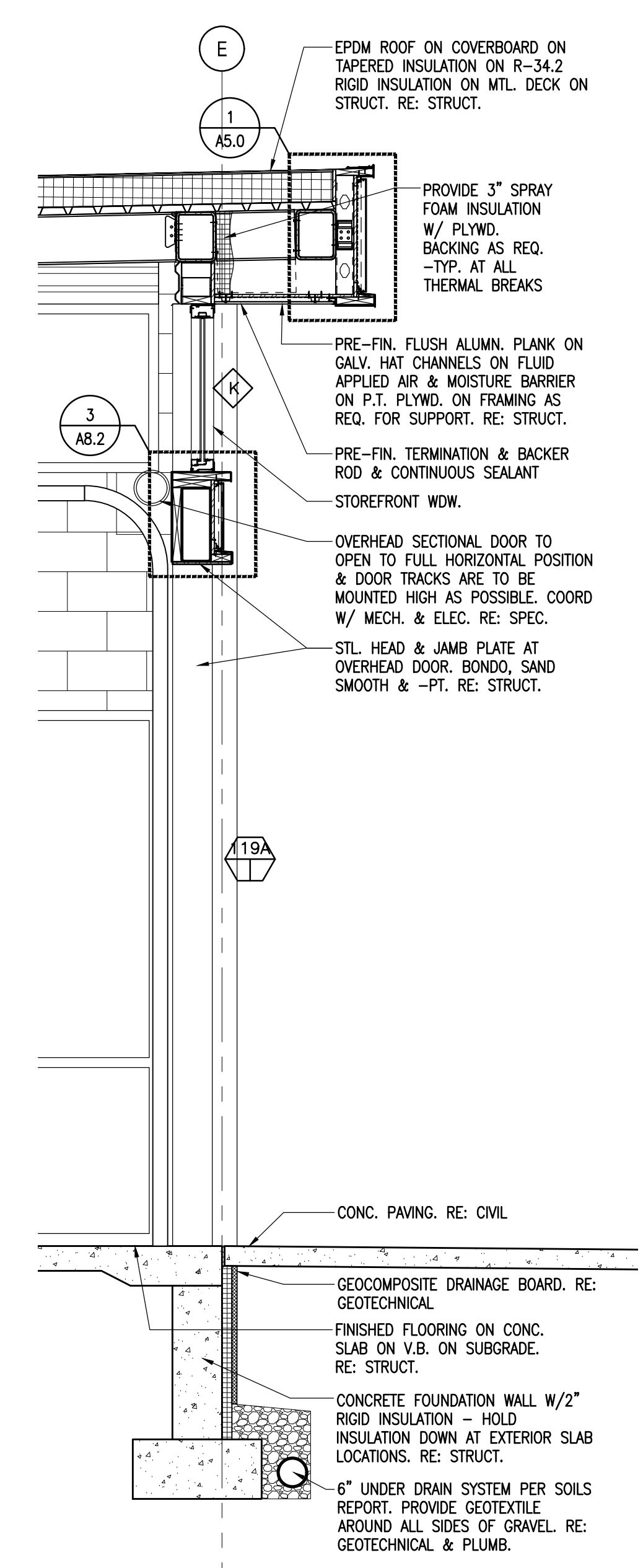
C BUILDING SECTION SCALE: 1/2"=1'-0"
