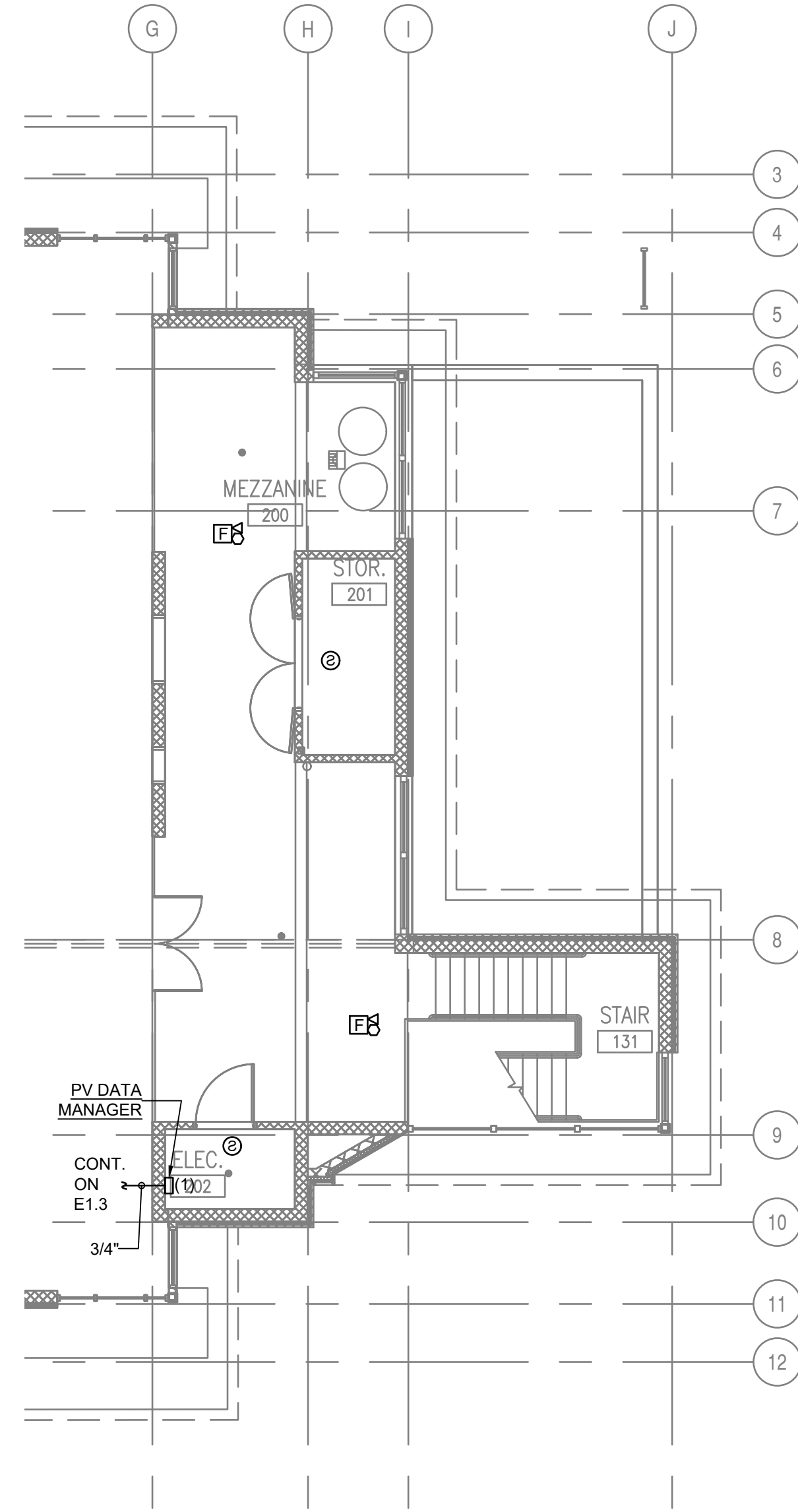
3 MEZZANINE SYSTEMS PLAN 1/8" = 1'-0"
