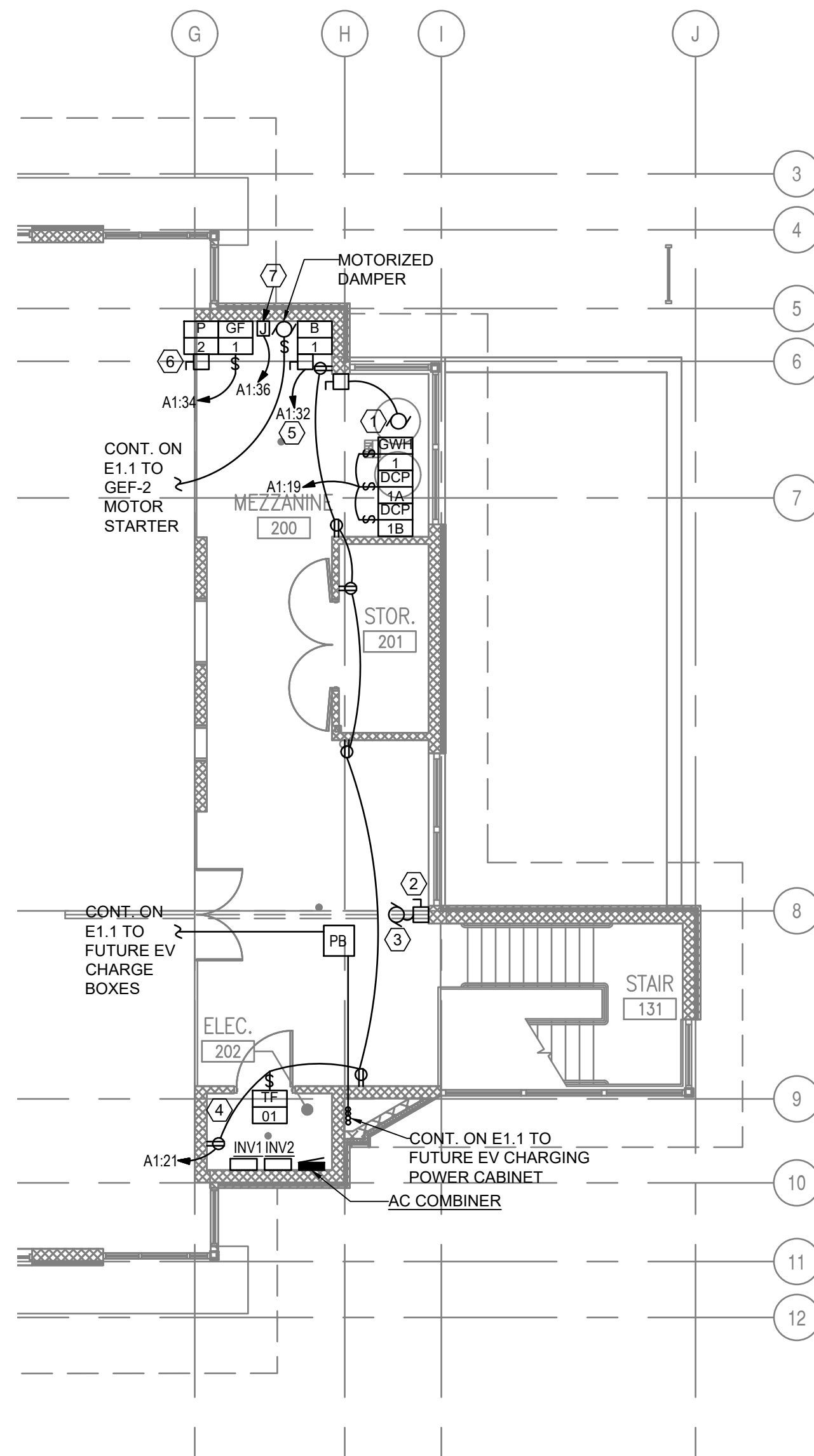
1 MEZZANINE POWER PLAN 1/8" = 1'-0"
