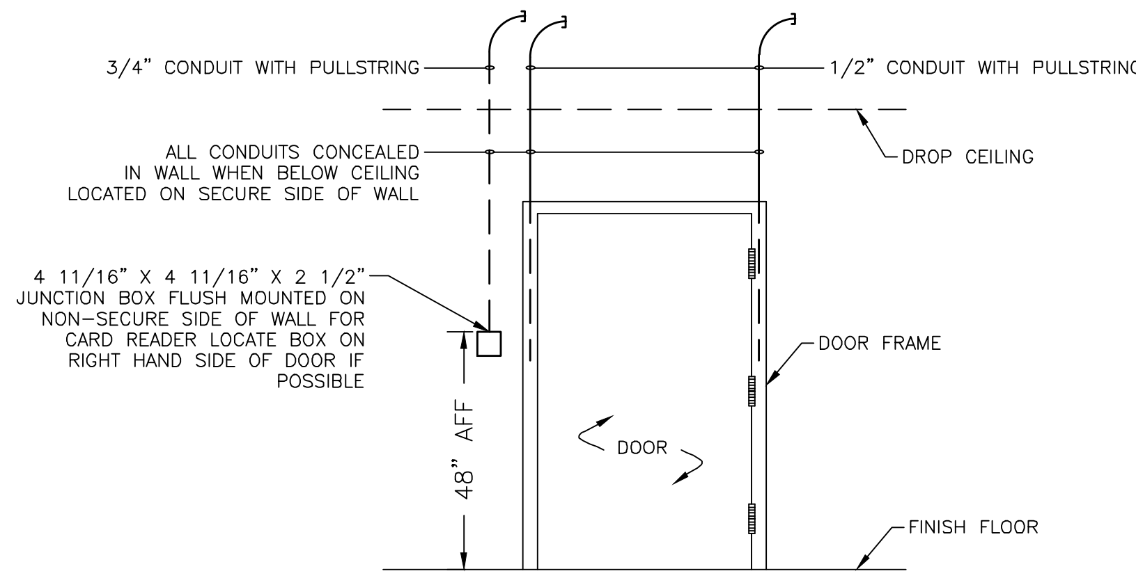
3 TYPICAL SECURITY DOOR ROUGH-IN (ACCESSIBLE CEILING) NO SCALE
