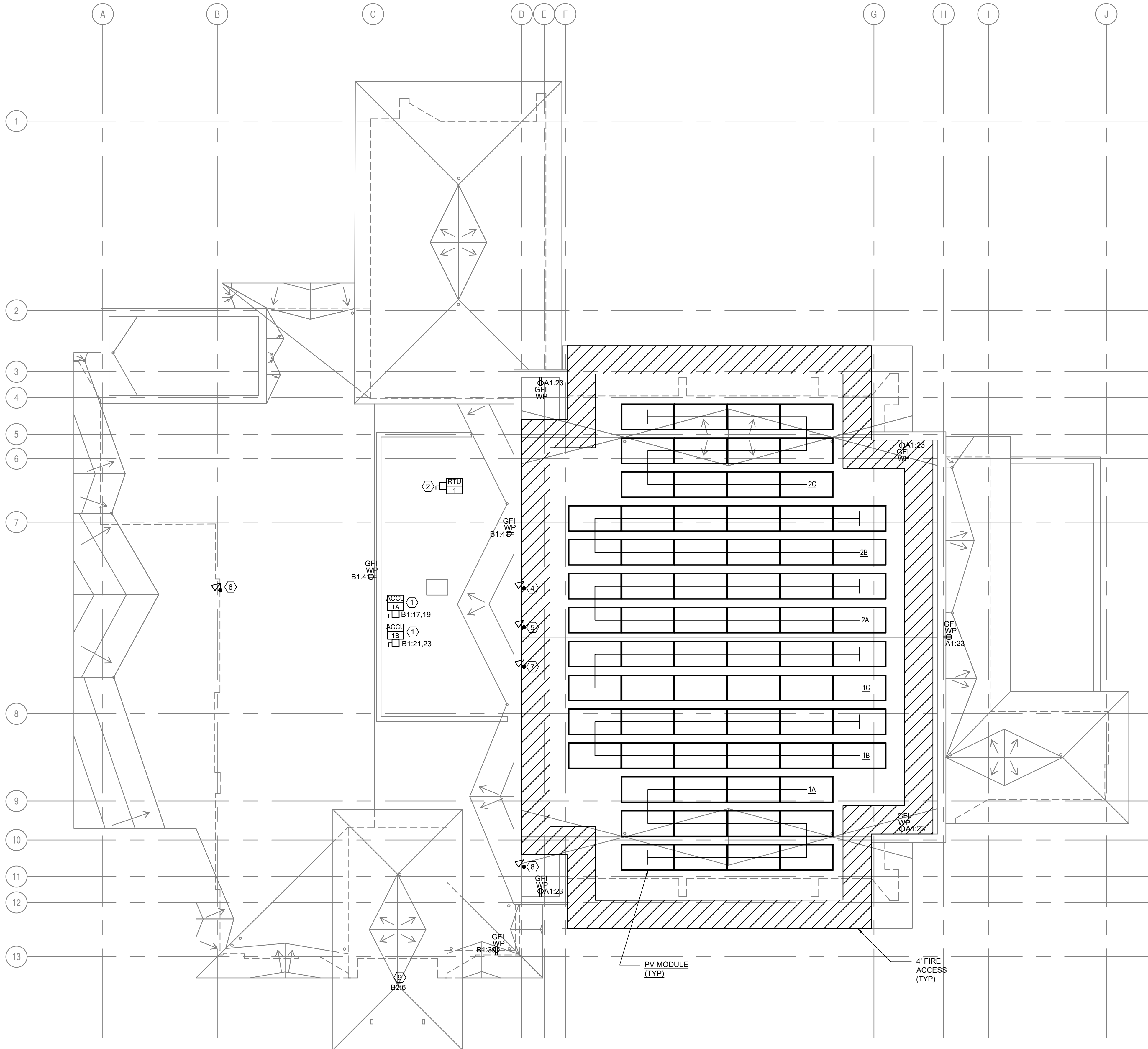
1 ROOF PLAN 1/8" = 1'-0"
