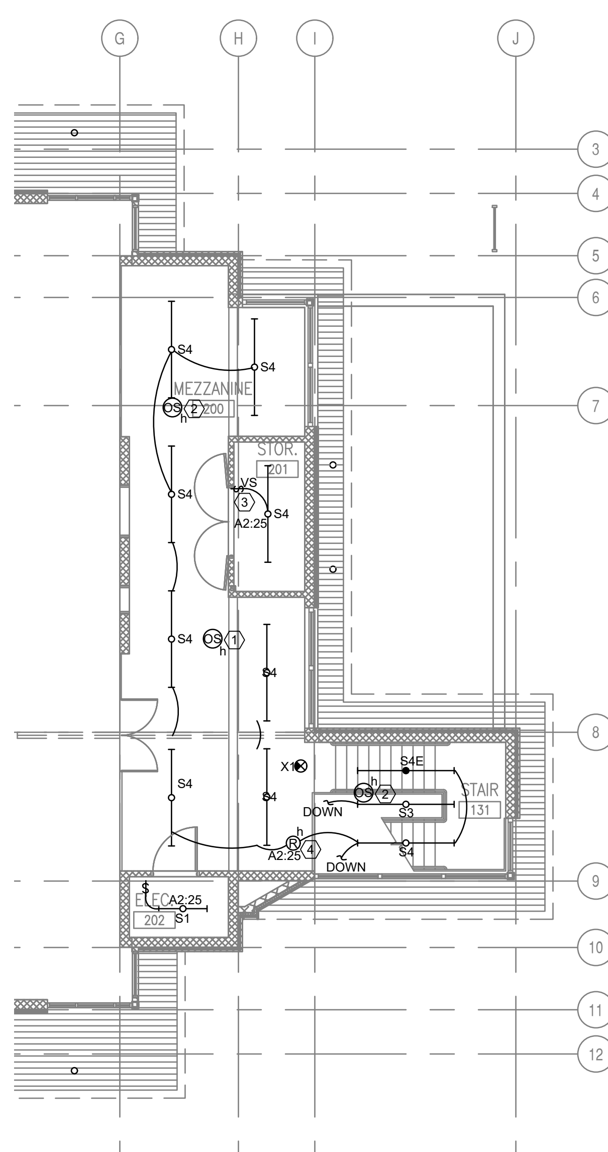
2 MEZZANINE LIGHTING PLAN 1/8" = 1'-0"
