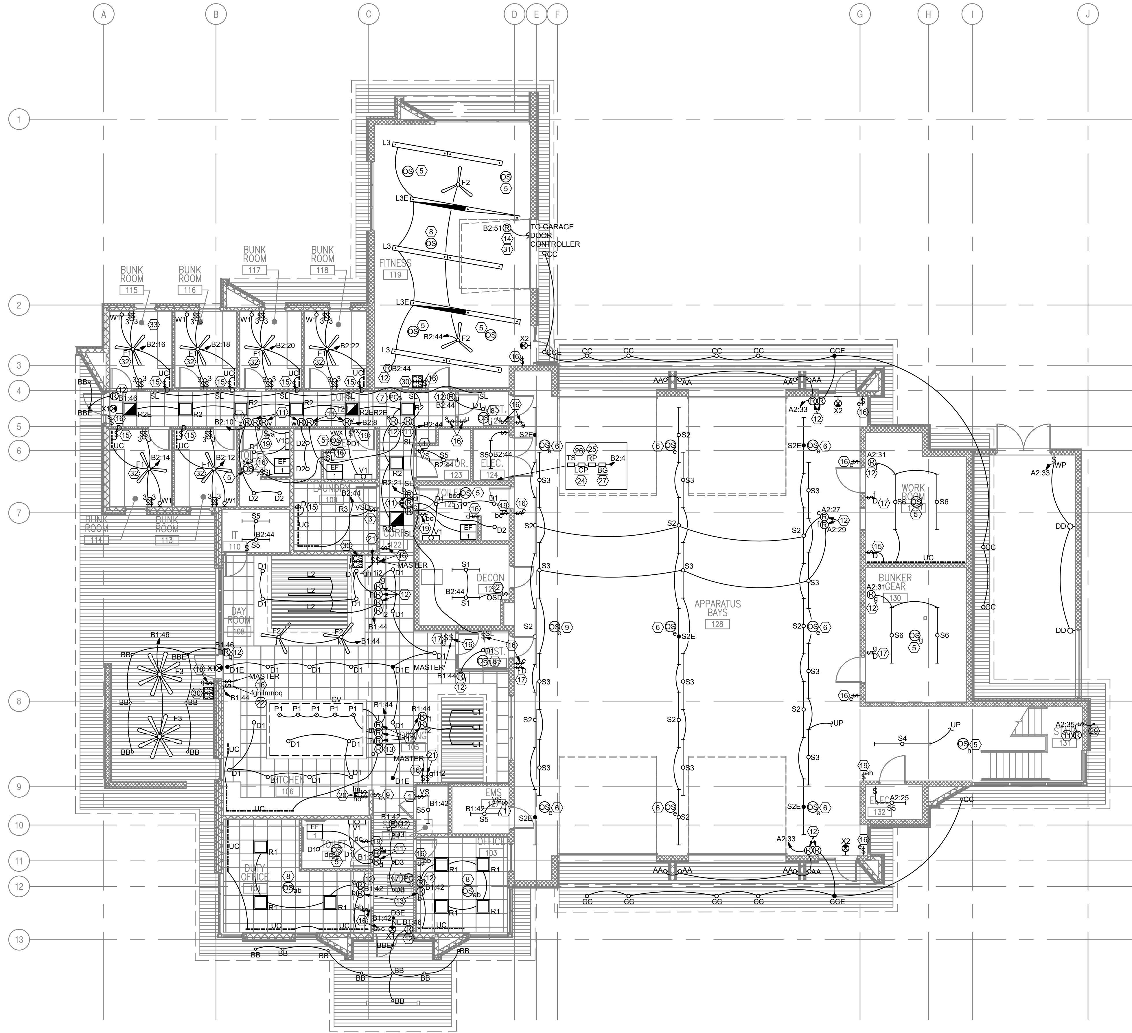
1 LIGHTING PLAN 1/8" = 1'-0"
