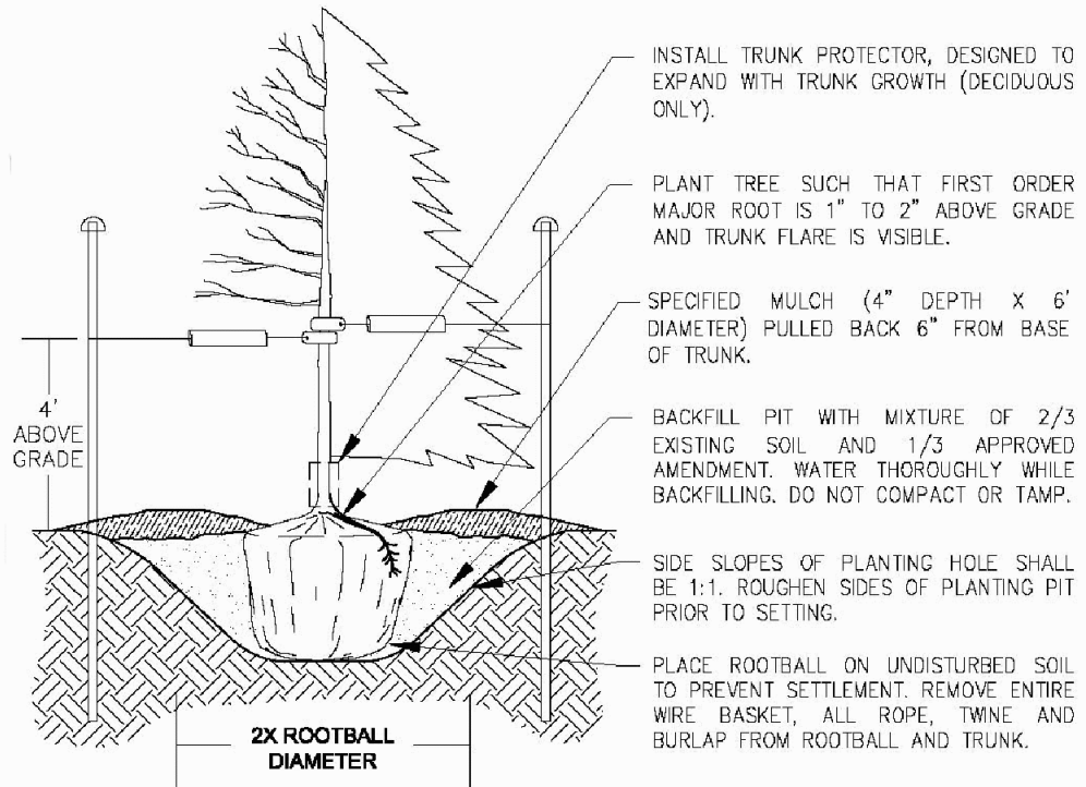
1 DECIDUOUS TREE PLANTING N.T.S.
