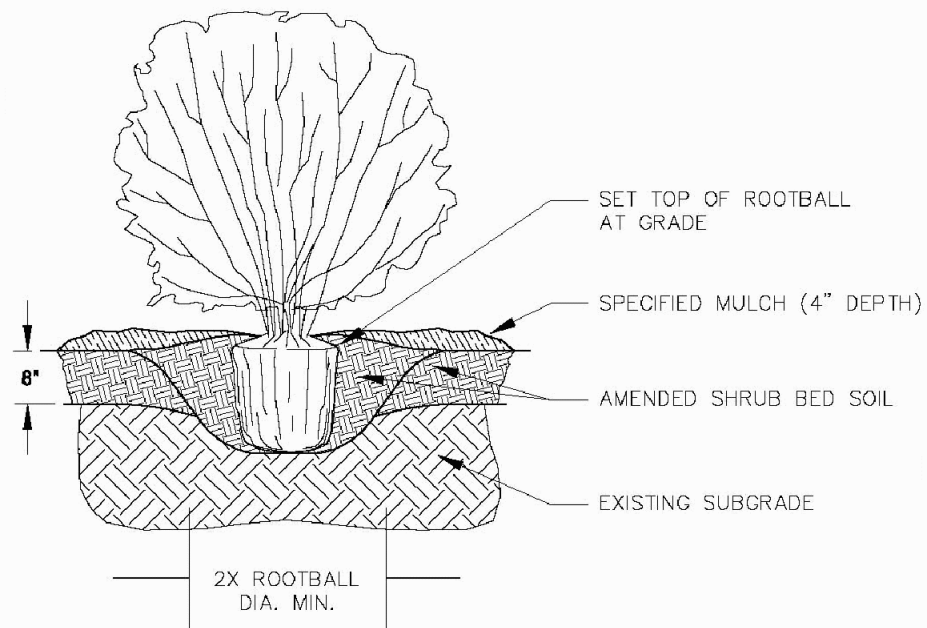
2 SHRUB PLANTING DETAIL N.T.S.
