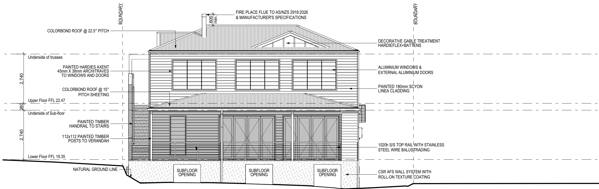
Rear Elevation - South Facing
