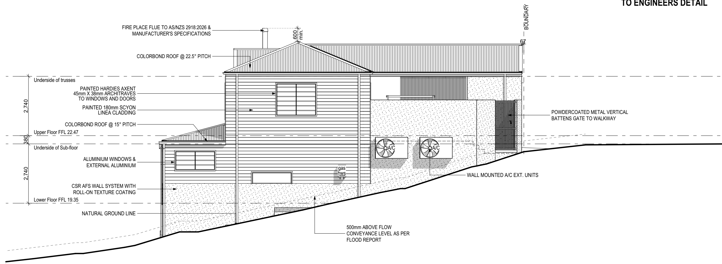
Left Elevation - East Facing
