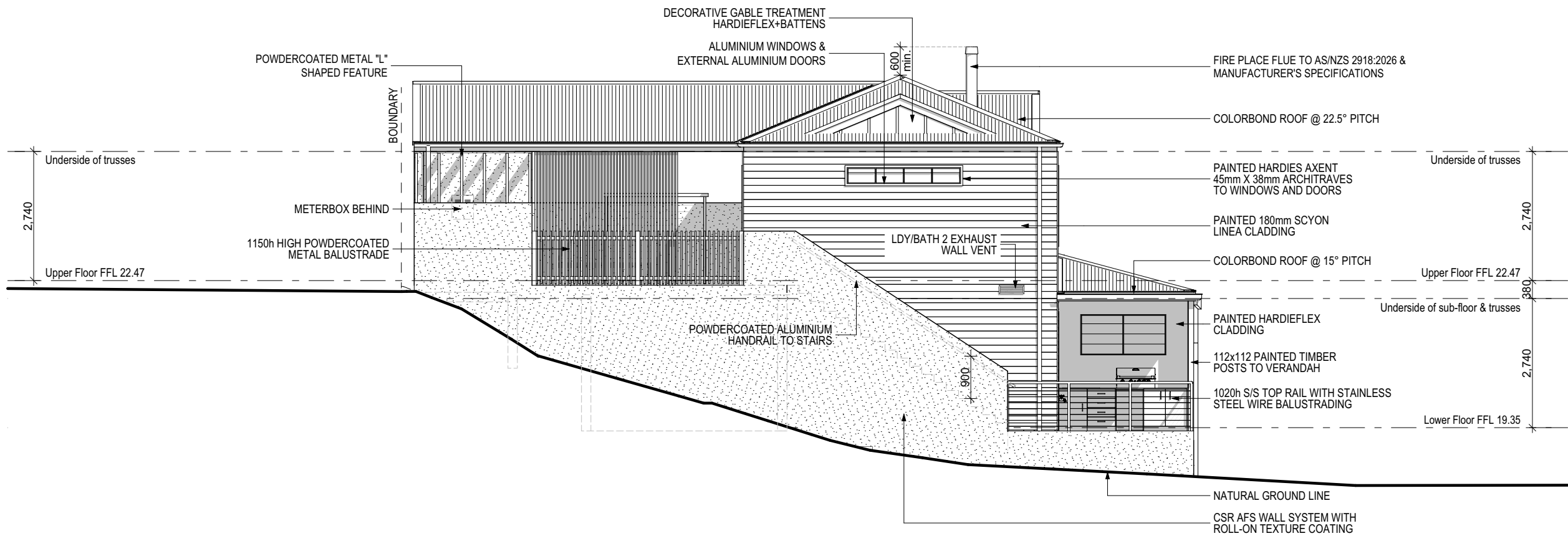
Right Elevation - West Facing
