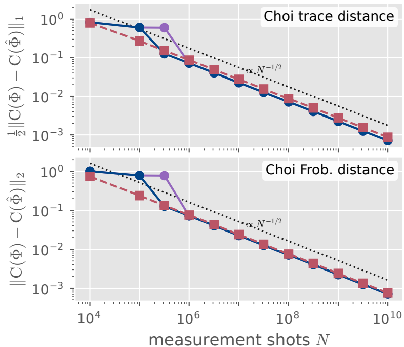
Accuracy vs. measurement shots
