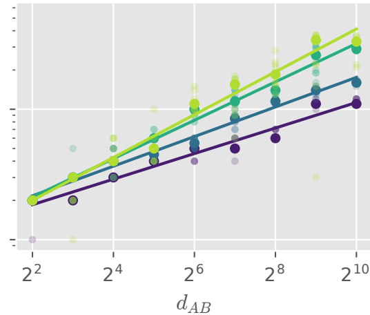
Choi rank d_{AB}
