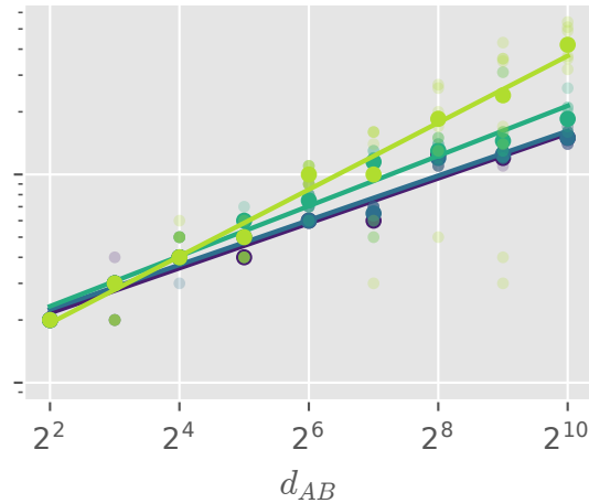
Choi rank \log_2 d_{AB}
