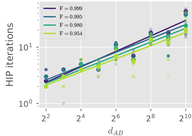
Choi rank 1 (isometry)
