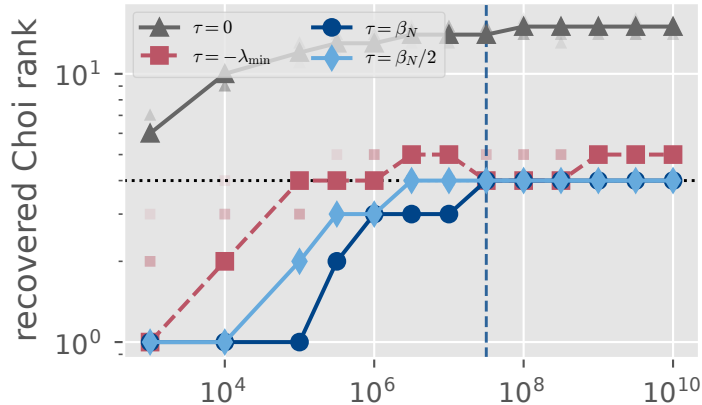
amplitude damping, d_{AB} = 2^6 , rank 4
