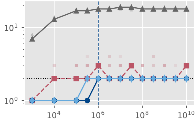
rank-2 channel, d_{AB} = 2^8
