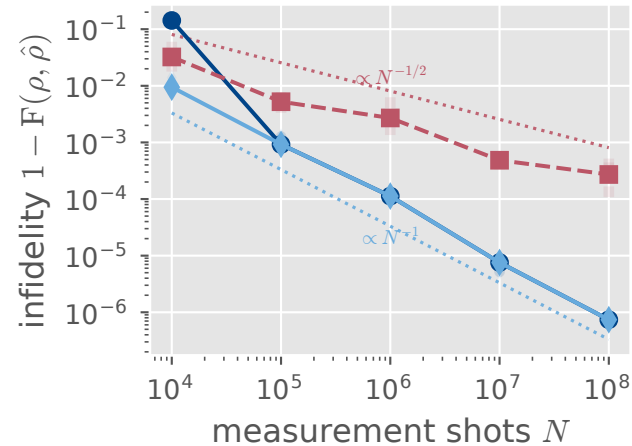
Choi infidelity
