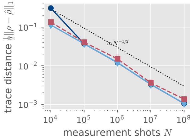
Choi trace distance
