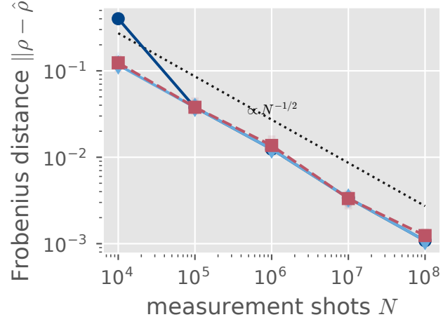
Choi Frobenius distance
