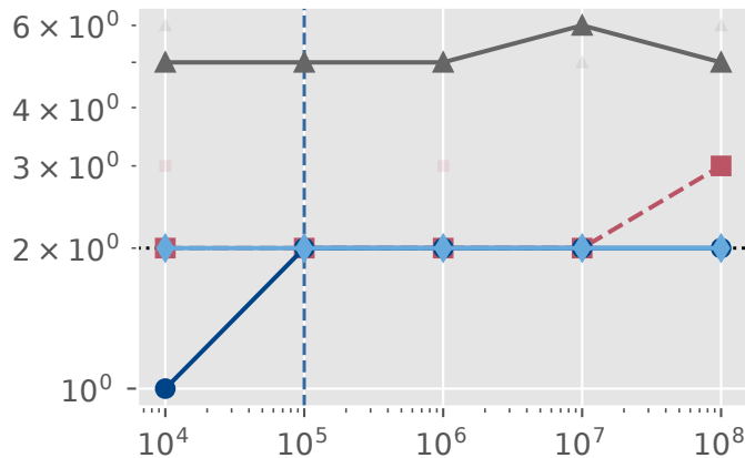
rank2, d_{AB} = 16
