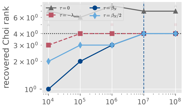
amp_damping_r2, d_{AB} = 16
