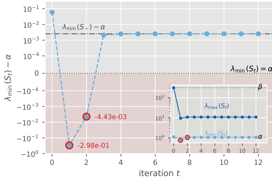
(b) transient exit from [\alpha, \beta] ( \kappa = 300 )
