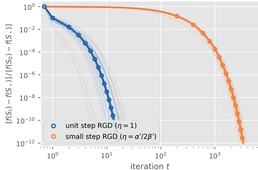
(a) unit against small step ( d = 2, n = 5, \kappa = 10^2 )
