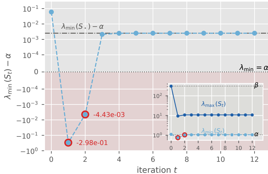
(b) transient exit from [\alpha I, \beta I] ( \kappa = 300 )
