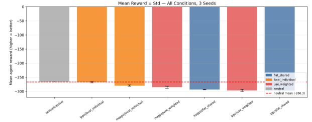
Fig. 5. Mean reward across all configurations with standard deviation over three seeds.
