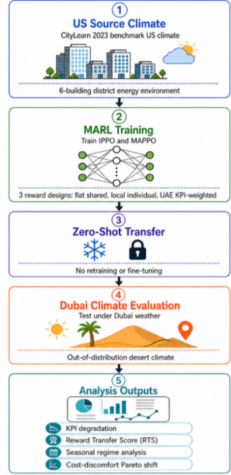
Fig. 1. Overview Of The Proposed MARL Reward Design Transferability Study
