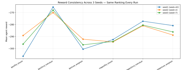
Fig. 6. Consistency of reward ranking across seeds.
