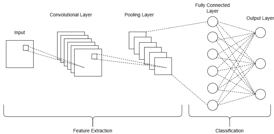
Figure 2.3: CNN Architecture
