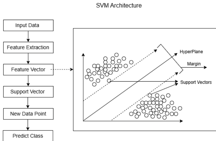
Figure 2.2: SVM Representation
