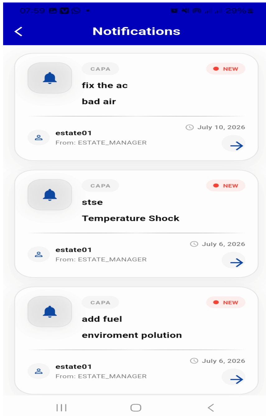
Figure 5.9: Notification Interface.
