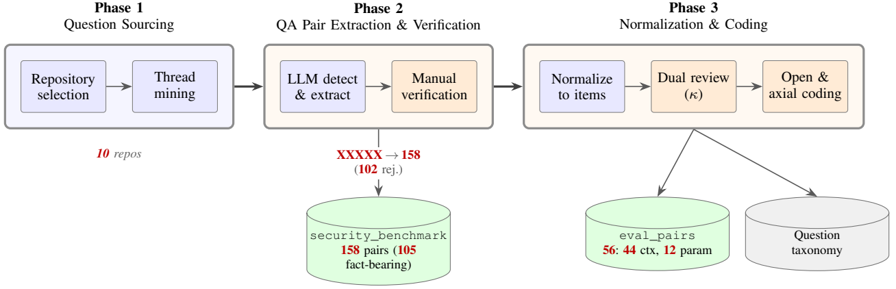
Fig. 1. SecDevQA construction pipeline. Three phases (§II-A–§II-C). Phase 1 sources candidate threads from 10 repositories; Phase 2 extracts candidate Q&A pairs with a two-stage LLM pipeline and screens them down to 158 human-verified pairs ( 105 stating an externally checkable hard fact); Phase 3 normalizes 56 pairs into self-contained, resolution-free evaluation items ( 44 contextual, 12 parametric) under independent dual annotation, and codes the corpus (open then axial) toward a question taxonomy. Blue steps are automated (LLM); orange steps are human-in-the-loop; green cylinders are released artifacts. Counts reflect the current state of construction and grow as the protocol is applied to more repositories.
