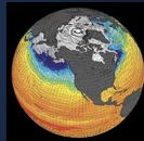
Climate change
