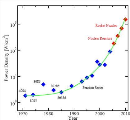
Evolution of selected microprocessors power density.
