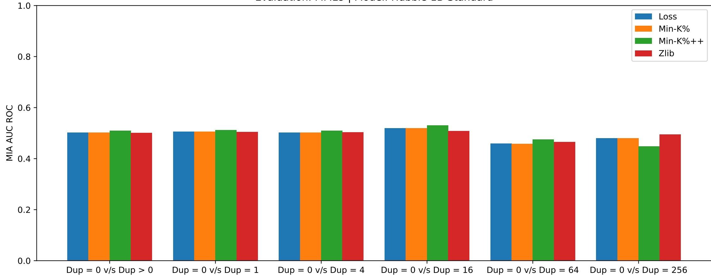
Evaluation: MMLU | Model: Hubble-1B-Standard
