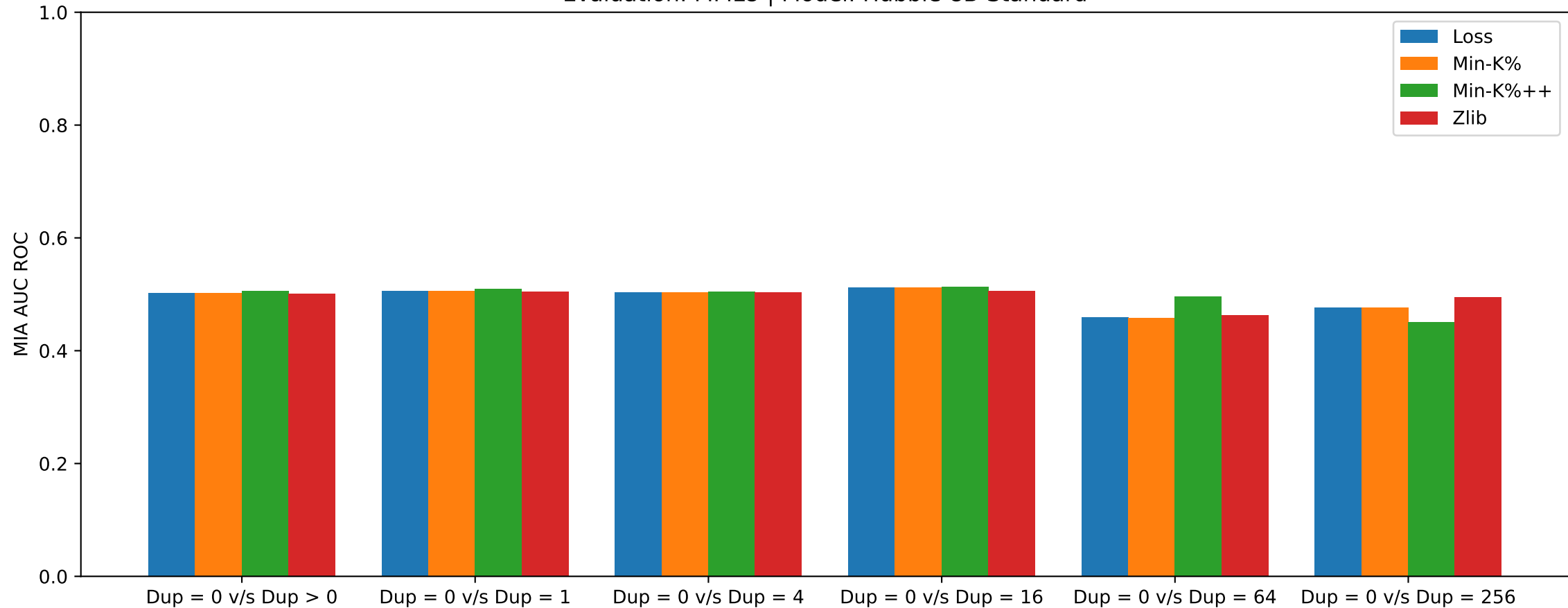
Evaluation: MMLU | Model: Hubble-8B-Standard
